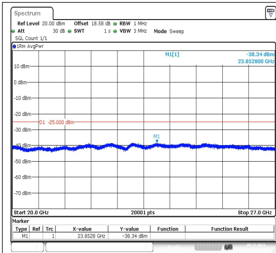
Band7_20MHz_QPSK_21350_1RB#0_20000~27000_000_20000~27000
