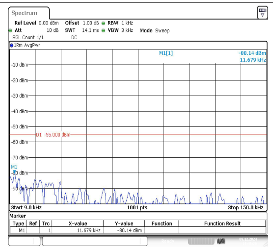
Band7_20MHz_16QAM_21350_1RB#0_0.009~0.15_5_0.009~0.15
