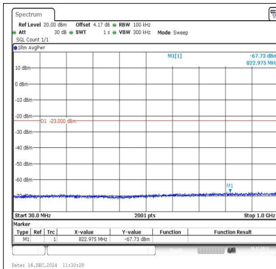
Band66_3MHz_QPSK_131987_1RB#0_30~1000_30~1000
