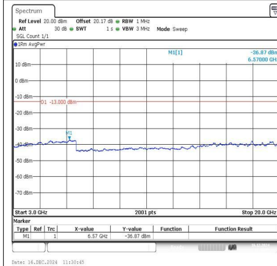
Band66_3MHz_QPSK_131987_1RB#0_3000~20000_000_3000~20000
