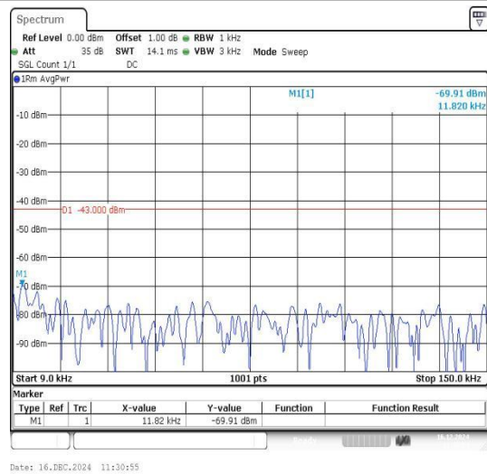
Band66_3MHz_16QAM_131987_1RB#0_0.009~0.15_15_0.009~0.15
