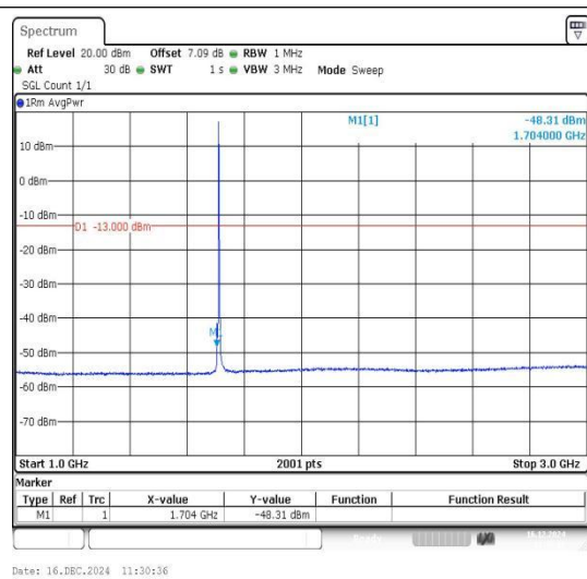
Band66_3MHz_QPSK_131987_1RB#0_1000~3000_0_1000~3000
