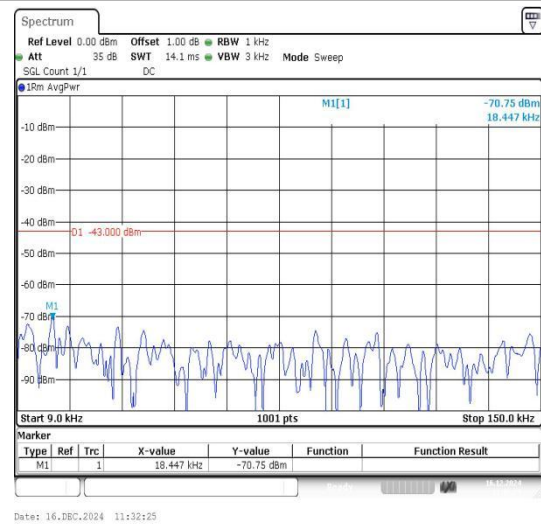
Band66_3MHz_16QAM_132322_1RB#0_0.009~0.15_0.009~0.15
