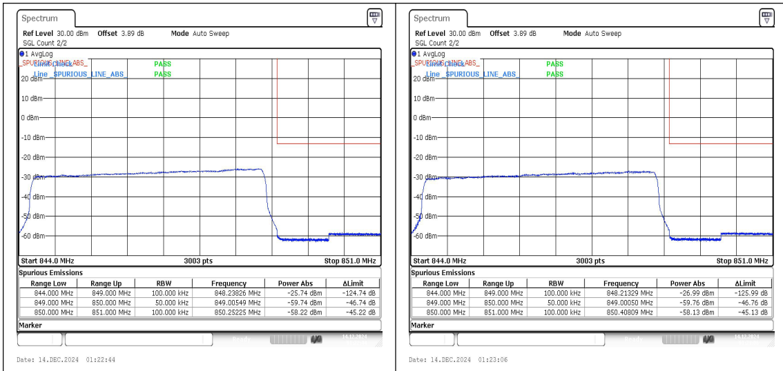
Band5_5MHz_QPSK_20625_25RB#0 Band5_5MHz_16QAM_20625_25RB#0
