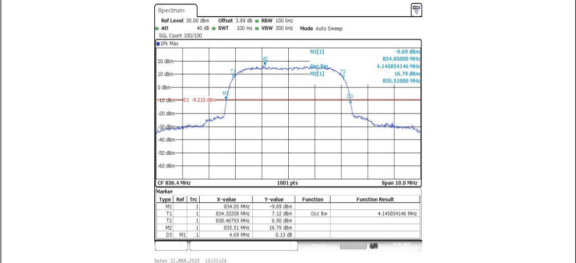
Band5-4182-2-PASS
