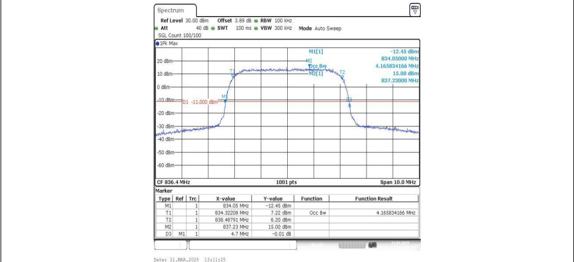
Band5-4182-1-PASS
