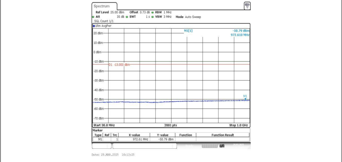
Band2-9400-4-30~1000MHz-PASS
