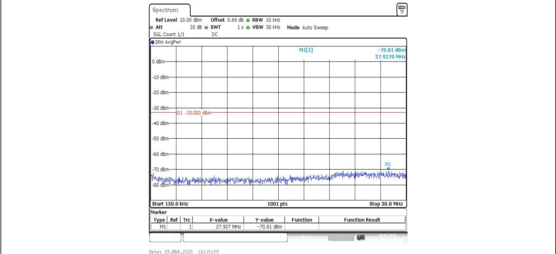
Band2-9262-5-0.15~30MHz-PASS
