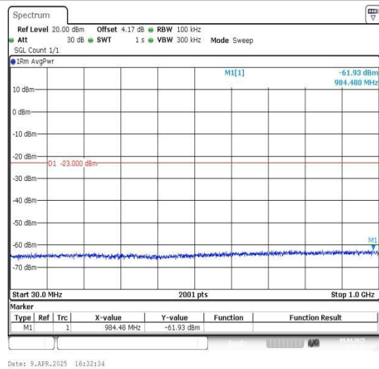
Band66_3MHz_16QAM_132657_1RB#0_30~1000_30~1000
