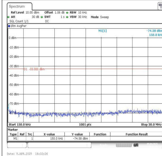
Band66_3MHz_16QAM_132657_1RB#0_0.15~30_0.15~30
