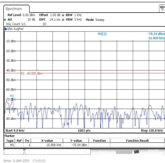
Band66_10MHz_16QAM_132022_1RB#0_0.009~0.15_0.009~0.15
