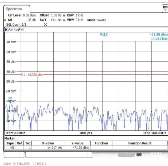
Band66_5MHz_16QAM_132647_1RB#0_0.009~0.15_0.009~0.15
