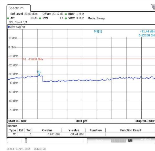
Band66_3MHz_QPSK_132657_1RB#0_3000~20000_3000~20000
