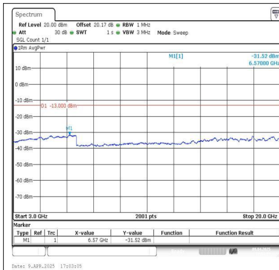
Band66_5MHz_QPSK_132647_1RB#0_3000~20000_3000~20000
