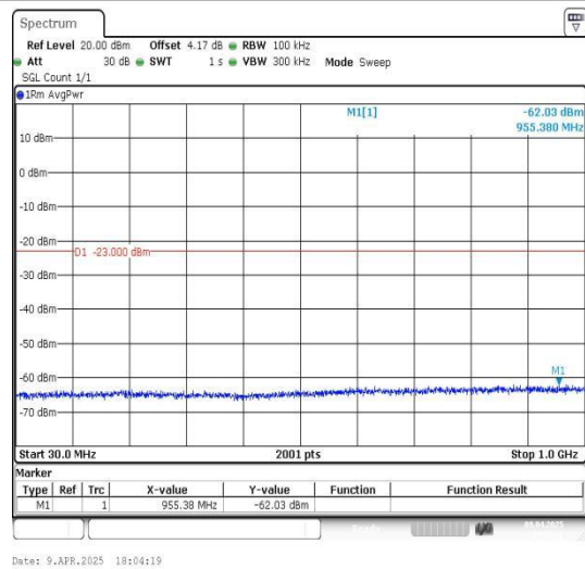
Band66_15MHz_16QAM_132597_1RB#0_30~1000_30~1000
