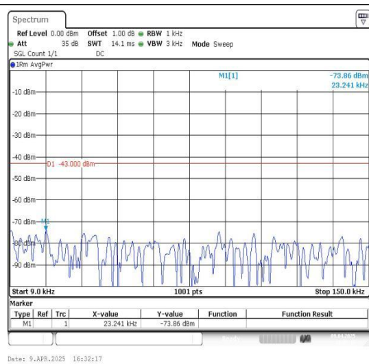
Band66_3MHz_16QAM_132657_1RB#0_0.009~0.15_0.009~0.15
