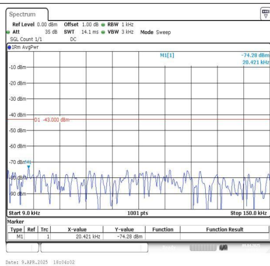
Band66_15MHz_16QAM_132597_1RB#0_0.009~0.15_0.009~0.15
