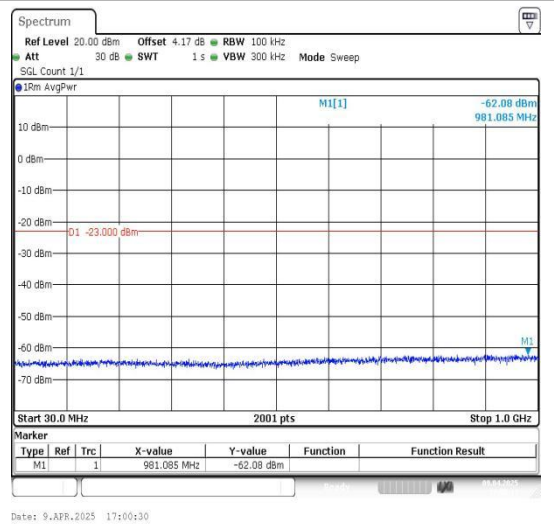
Band66_5MHz_16QAM_131997_1RB#0_30~1000_30~1000
