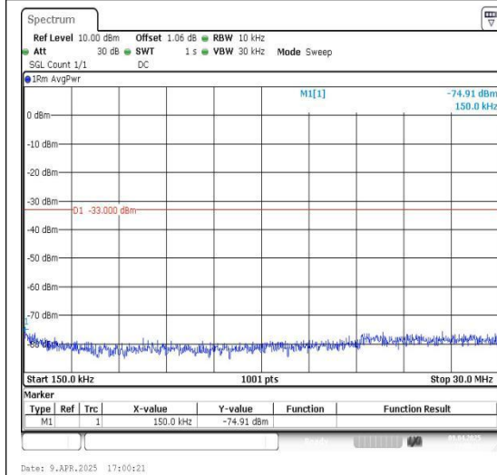
Band66_5MHz_16QAM_131997_1RB#0_0.15~30_0.15~30
