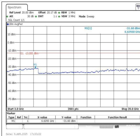
Band66_10MHz_QPSK_132022_1RB#0_3000~20000_3000~20000
