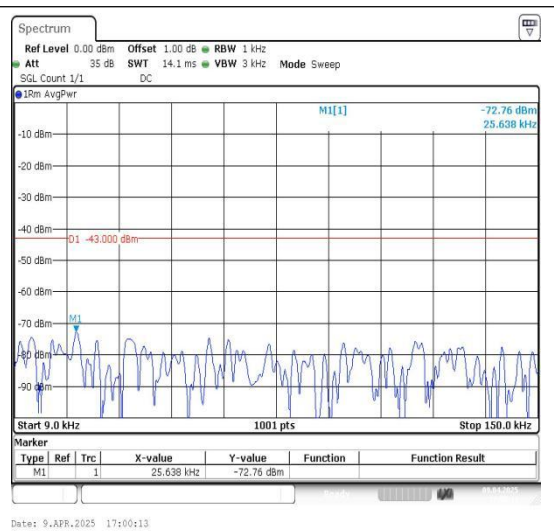
Band66_5MHz_16QAM_131997_1RB#0_0.009~0.15_0.009~0.15
