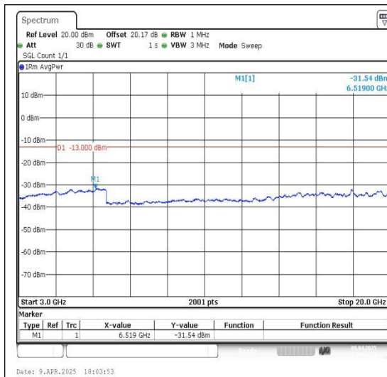
Band66_15MHz_QPSK_132597_1RB#0_3000~20000_3000~20000
