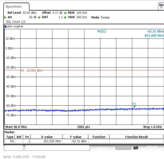
Band66_10MHz_16QAM_132022_1RB#0_0.30~1.0_0.30~1000
