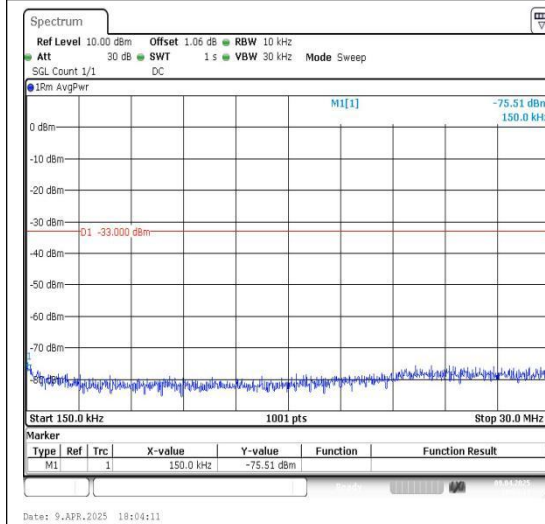
Band66_15MHz_16QAM_132597_1RB#0_0.15~30_0.15~30
