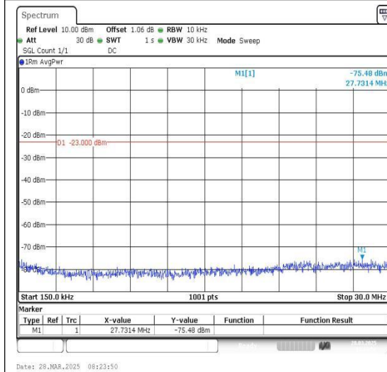
Band12_5MHz_16QAM_23095_1RB#0_0.15~30_0.15~30
