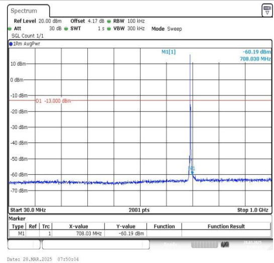
Band12_3MHz_16QAM_23025_1RB#0_30~1000_30~1000
