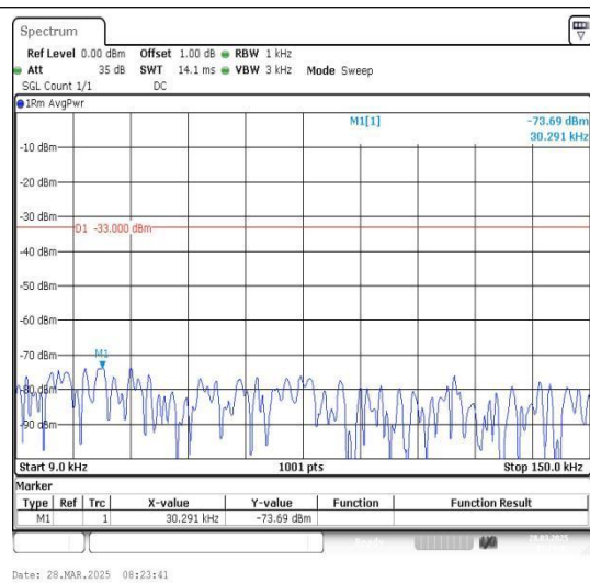
Band12_5MHz_16QAM_23095_1RB#0_0.009~0.15_0.009~0.15
