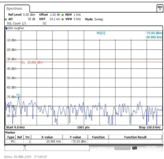
Band12_3MHz_16QAM_23025_1RB#0_0.009~0.15_0.009~0.15
