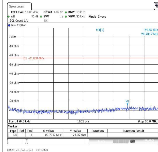
Band12_5MHz_16QAM_23035_1RB#0_0.15~30_0.15~30
