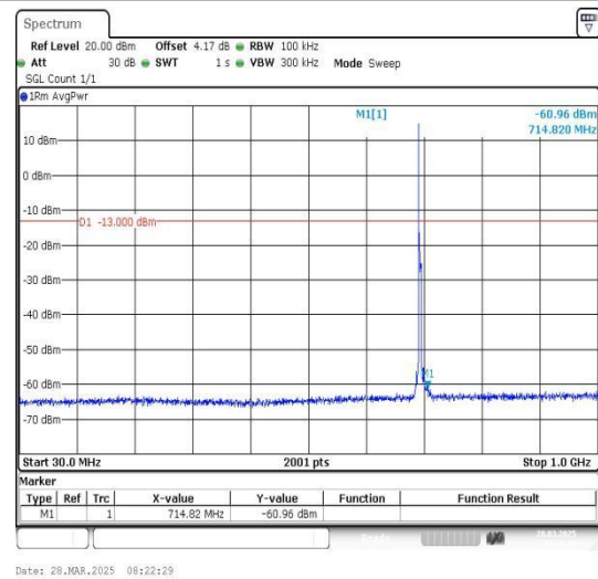
Band12_5MHz_16QAM_23035_1RB#0_30~1000_30~1000
