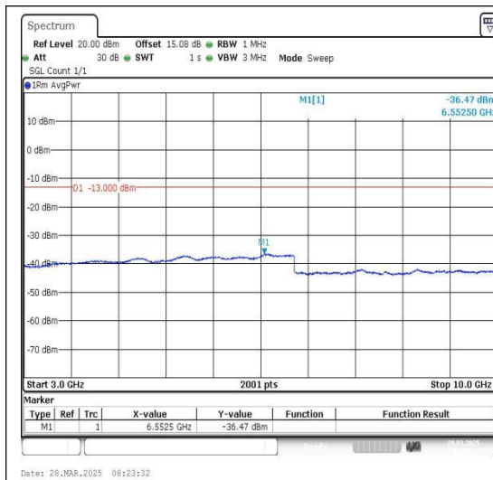
Band12_5MHz_QPSK_23095_1RB#0_3000~10000_3000~10000
