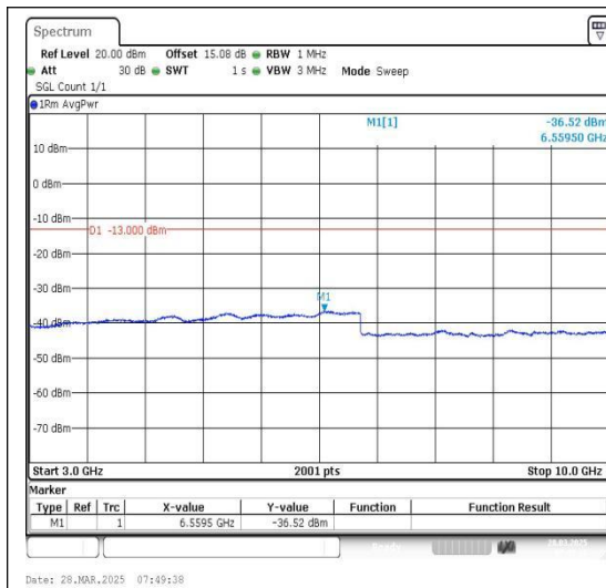
Band12_3MHz_QPSK_23025_1RB#0_3000~10000_3000~10000
