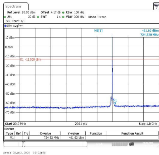
Band12_5MHz_16QAM_23095_1RB#0_30~1000_30~1000
