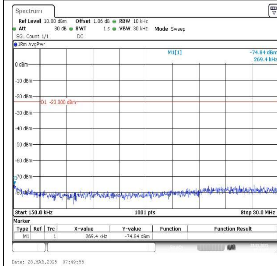
Band12_3MHz_16QAM_23025_1RB#0_0.15~30_0.15~30
