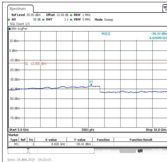
Band12_5MHz_QPSK_23035_1RB#0_3000~10000_3000~10000
