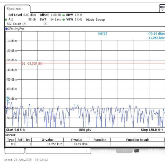
Band12_5MHz_16QAM_23035_1RB#0_0.009~0.15_0.009~0.15
