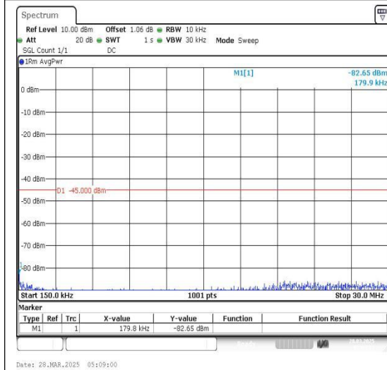
Band7_5MHz_QPSK_20775_1RB#0_0.15~30_0.15~30
