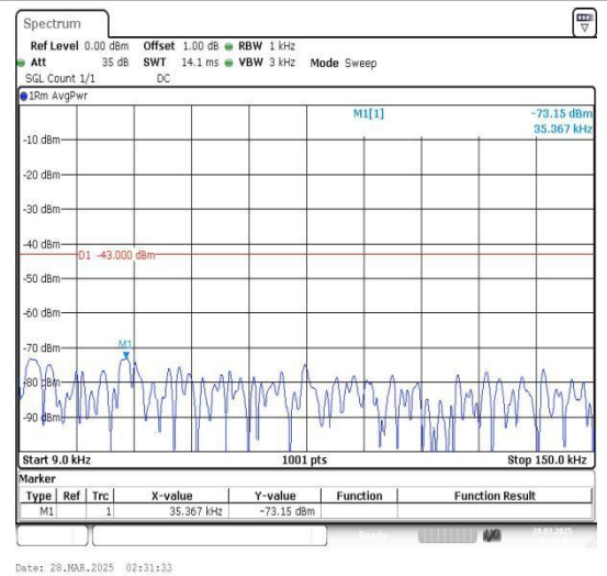
Band4_20MHz_16QAM_20175_1RB#0_0.009~0.15_0.009~0.15
