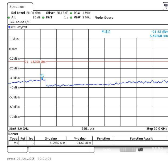
Band4_20MHz_QPSK_20175_1RB#0_3000~20000_3000~20000
