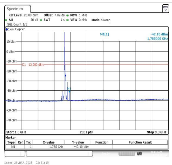
Band4_20MHz_QPSK_20175_1RB#0_1000~3000_1000~3000
