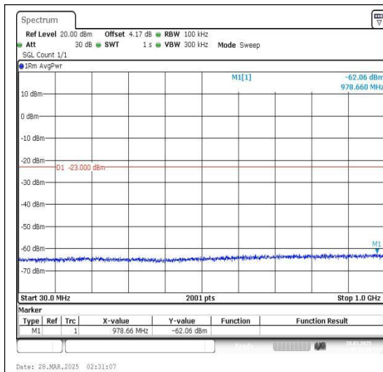
Band4_20MHz_QPSK_20175_1RB#0_30~1000_30~1000
