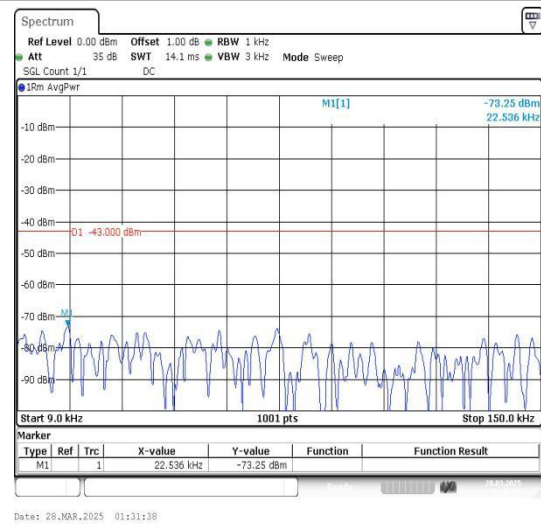
Band4_10MHz_16QAM_20350_1RB#0_0.009~0.15_0.009~0.15
