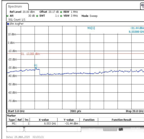
Band4_15MHz_QPSK_20175_1RB#0_3000~20000_3000~20000
