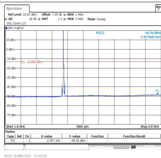
Band4_10MHz_QPSK_20350_1RB#0_1000~3000_1000~3000
