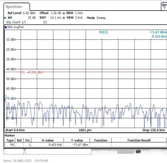
Band4_5MHz_16QAM_20175_1RB#0_0.009~0.15_0.009~0.15
