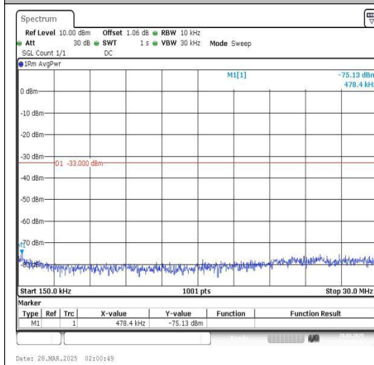
Band4_15MHz_QPSK_20175_1RB#0_3000~20000_3000~20000
