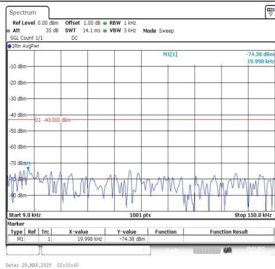
Band4_15MHz_16QAM_20175_1RB#0_0.009~0.15_0.009~0.15
