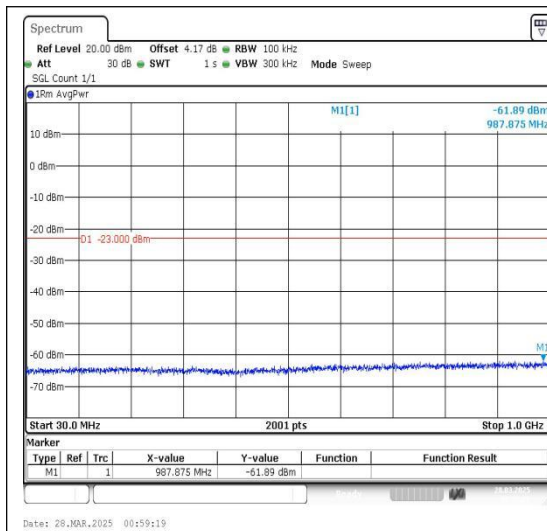
Band4_5MHz_QPSK_20175_1RB#0_30~1000_3 0~1000
