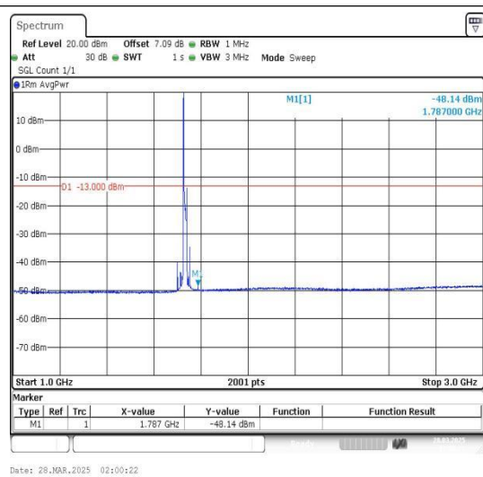
Band4_15MHz_QPSK_20175_1RB#0_1000~3000_1000~3000
