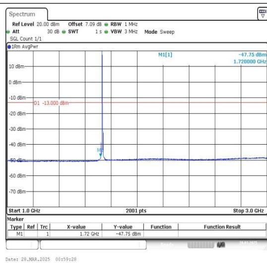
Band4_5MHz_QPSK_20175_1RB#0_1000~3000_1000~3000
