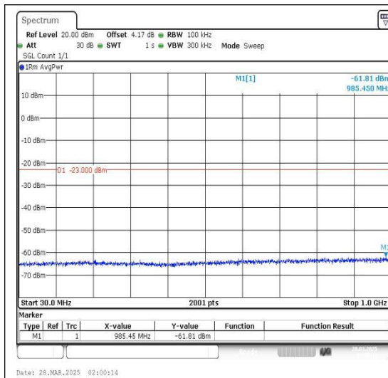
Band4_15MHz_QPSK_20175_1RB#0_30~1000_30~1000
