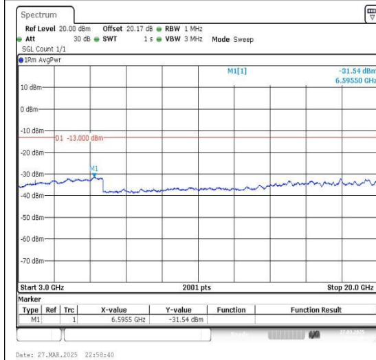
Band2_15MHz_QPSK_19125_1RB#0_3000~20000_3000~20000
