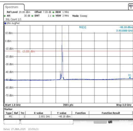
Band2_15MHz_QPSK_19125_1RB#0_1000~3000_1000~3000
