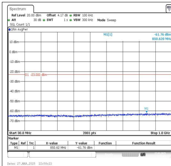
Band2_15MHz_QPSK_19125_1RB#0_30~1000_30~1000
