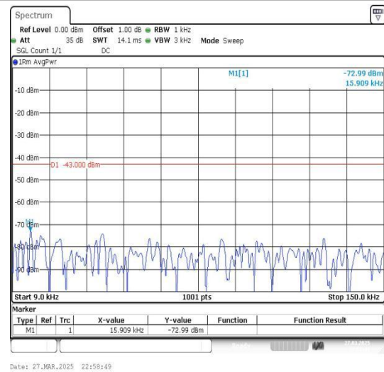
Band2_15MHz_16QAM_19125_1RB#0_0.009~0.15_0.009~0.15
