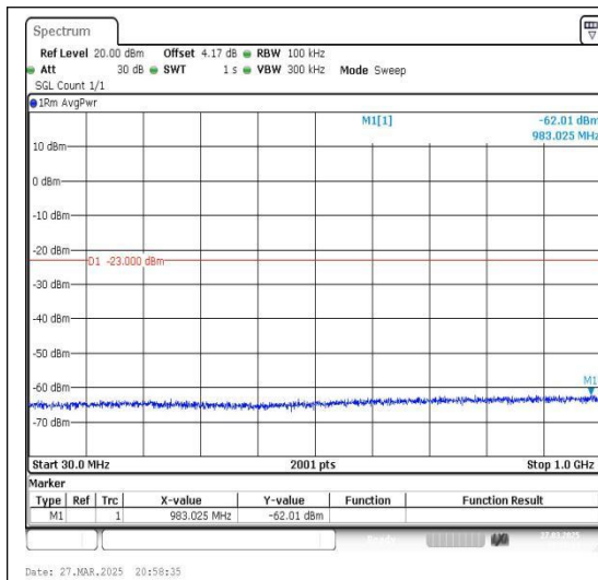
Band2_1.4MHz_QPSK_19193_1RB#0_30~1000_30~1000
