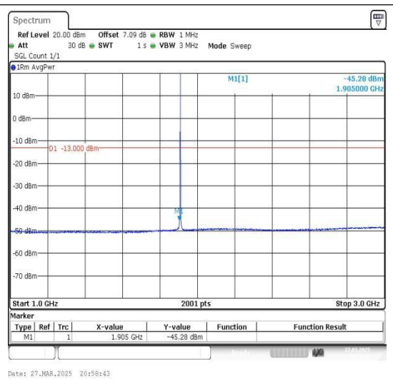
Band2_1.4MHz_QPSK_19193_1RB#0_1000~3000_0_1000~3000
