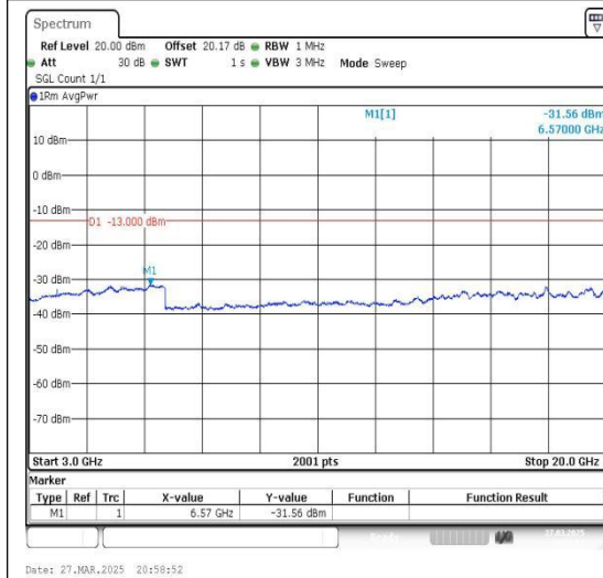
Band2_1.4MHz_QPSK_19193_1RB#0_3000~20000_00_3000~20000
