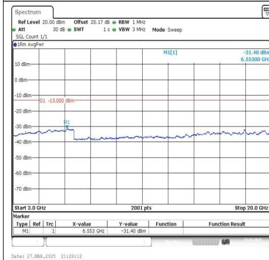
Band2_3MHz_QPSK_19185_1RB#0_3000~2000_0_3000~20000
