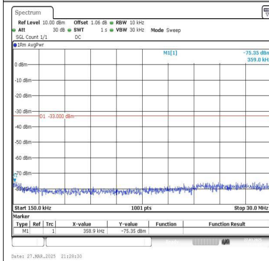
Band2_3MHz_QPSK_19185_1RB#0_3000~2000_0_3000~20000
