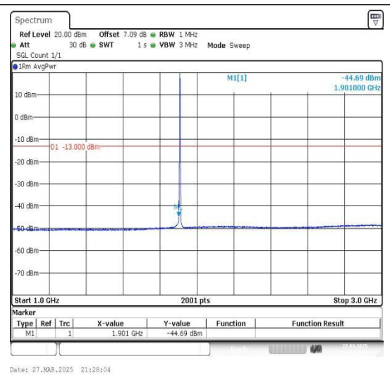
Band2_3MHz_QPSK_19185_1RB#0_1000~3000_1000~3000
