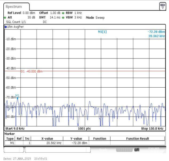
Band2_1.4MHz_16QAM_19193_1RB#0_0.009~0.15_0.009~0.15
