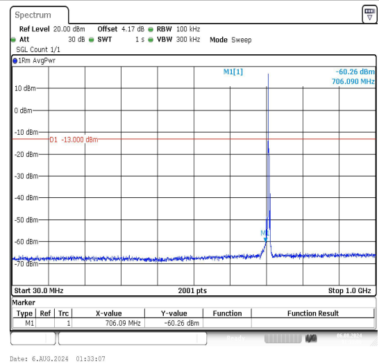
Band12_3MHz_16QAM_23165_1RB#0_30~1000_ 30~1000
