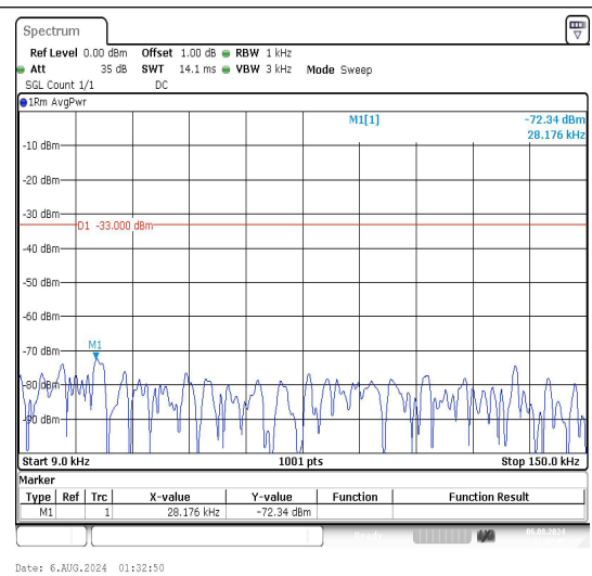
Band12_3MHz_16QAM_23165_1RB#0_0.009~0.1 5_0.009~0.15
