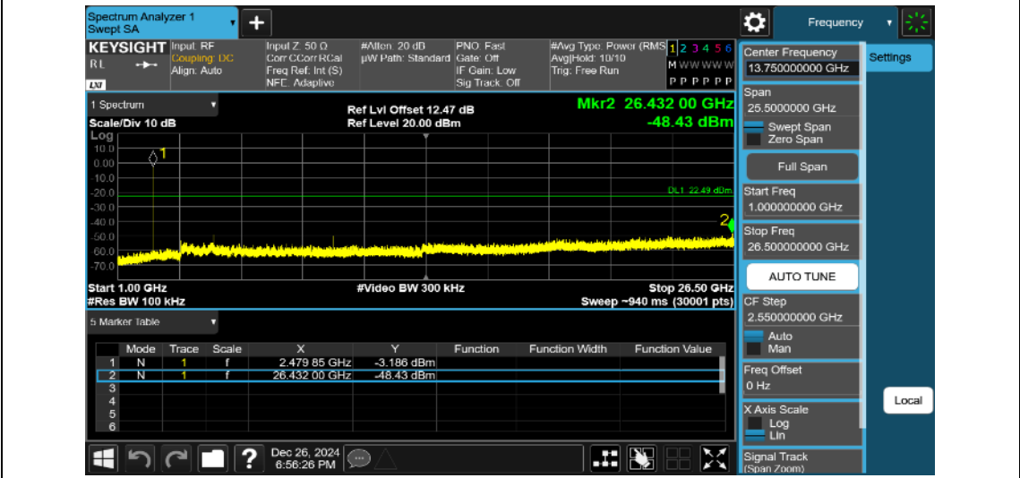
DH5-Ant1-2480-1000~26500-PASS
