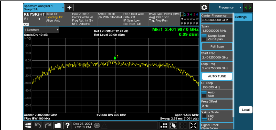
3DH5-Ant1-2402-0~Reference-PASS
