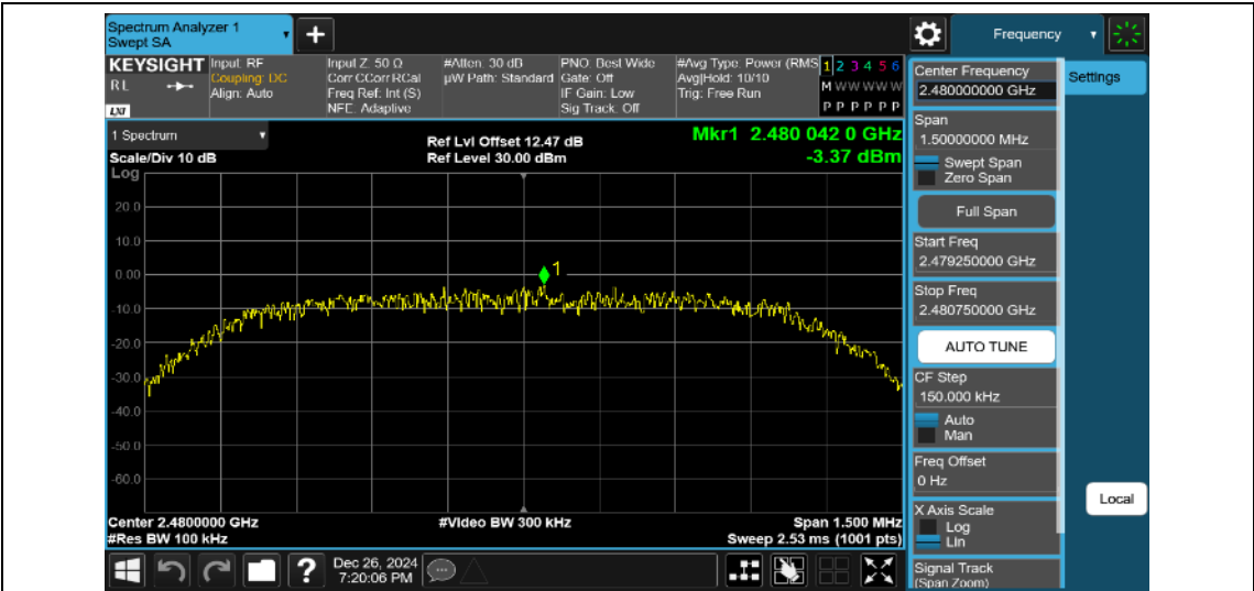
2DH5-Ant1-2480-0~Reference-PASS
