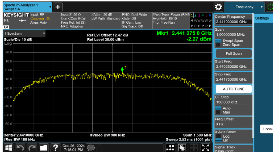
2DH5-Ant1-2441-0~Reference-PASS
