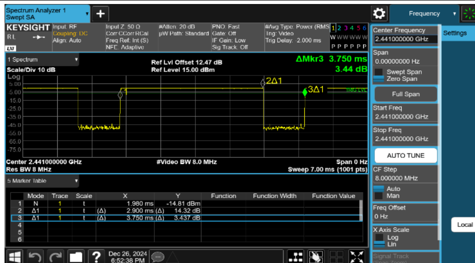
NTNV-DH5-Ant1-2441
