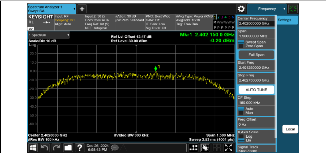
2DH5-Ant1-2402-0~Reference-PASS
