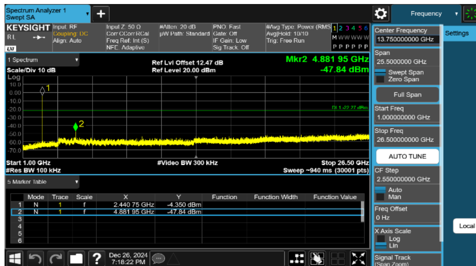
2DH5-Ant1-2441-1000~26500-PASS
