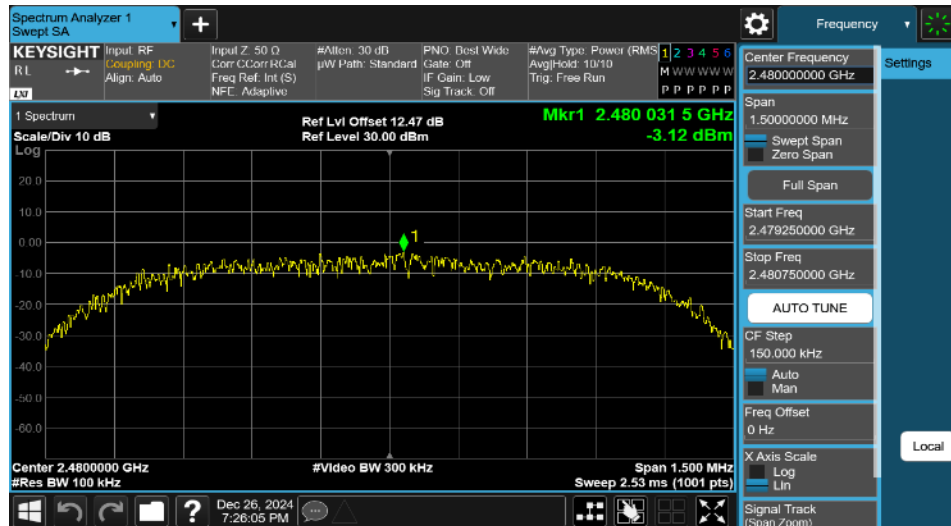
3DH5-Ant1-2480-0~Reference-PASS
