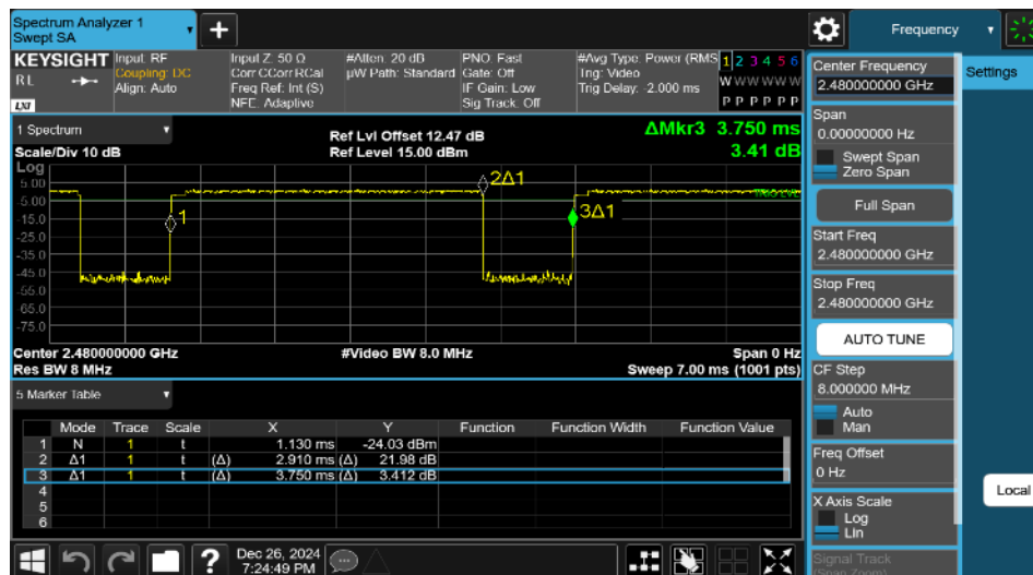
NTNV-3DH5-Ant1-2480
