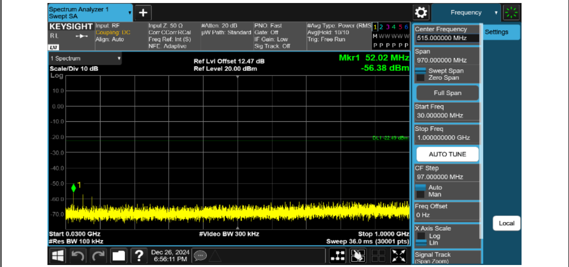
DH5-Ant1-2480-30~1000-PASS
