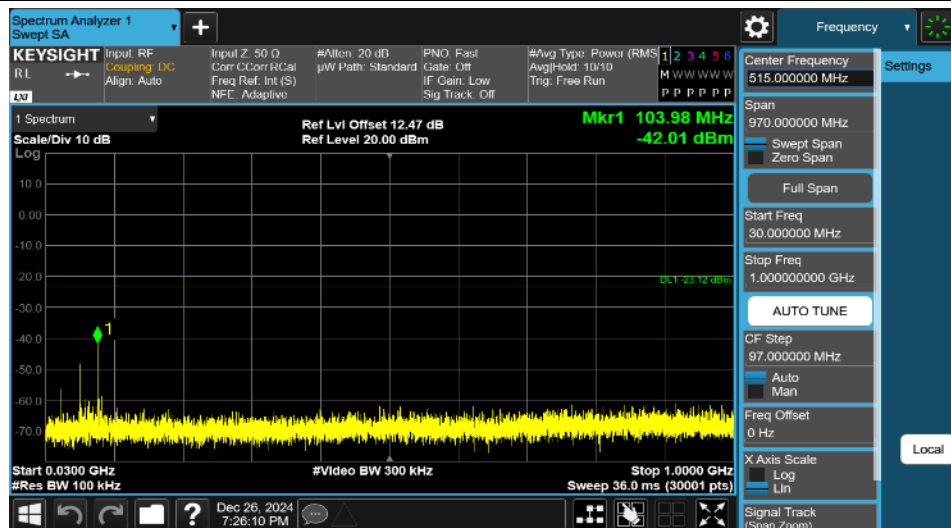
3DH5-Ant1-2480-30~1000-PASS
