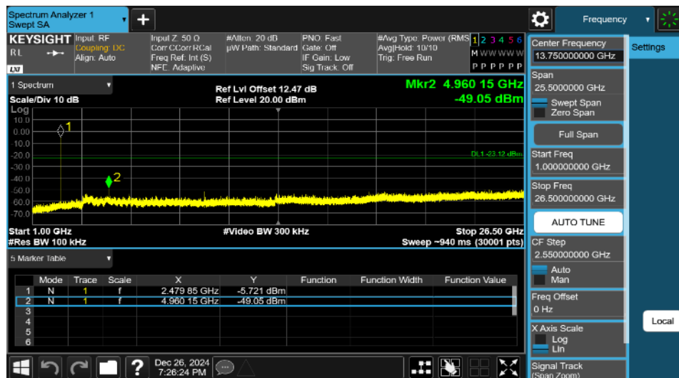
3DH5-Ant1-2480-1000~26500-PASS
