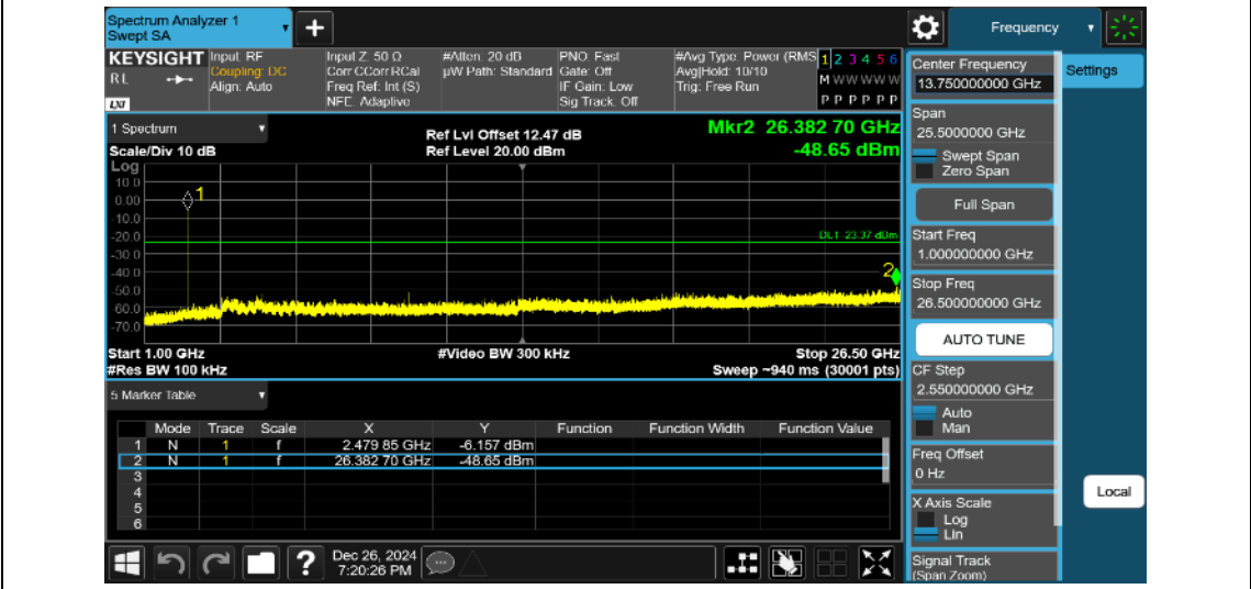
2DH5-Ant1-2480-1000~26500-PASS
