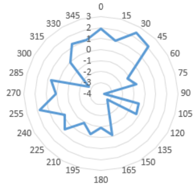
Ant2
