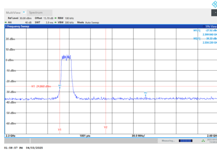
Bandedge-CH01
