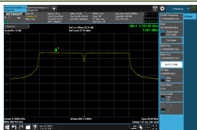
Channel 159 (5795MHz)
