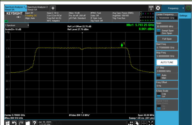
Channel 157 (5785MHz)
