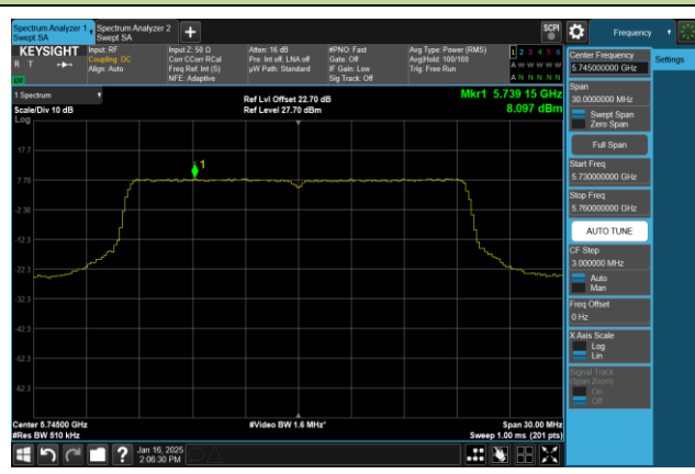
Channel 149 (5745MHz)
