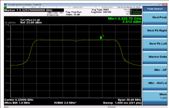
Channel 64 (5320MHz)
