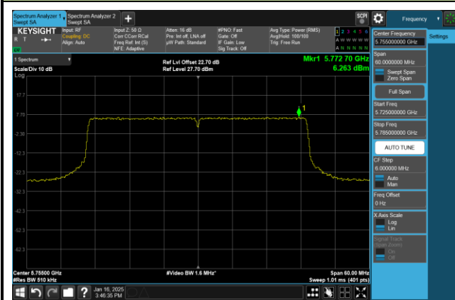
Channel 151 (5755MHz)
