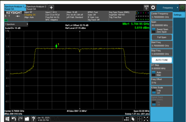
Channel 159 (5795MHz)
