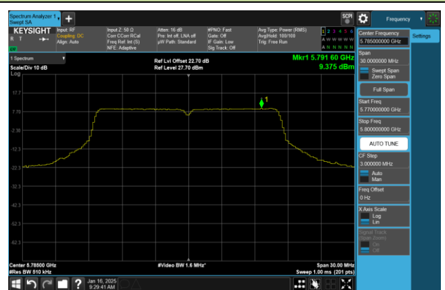
Channel 157 (5785MHz)
