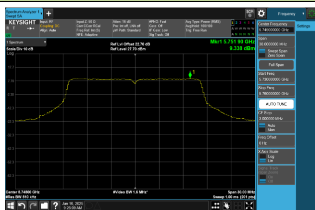
Channel 149 (5745MHz)
