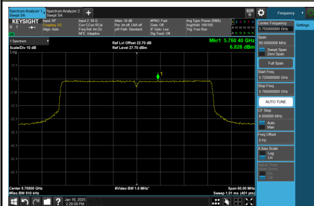
Channel 151 (5755MHz)
