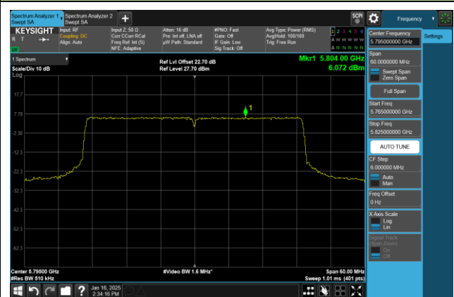
Channel 159 (5795MHz)
