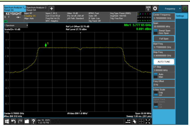
Channel 157 (5785MHz)
