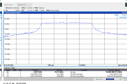
99 % Occupied Bandwidth
