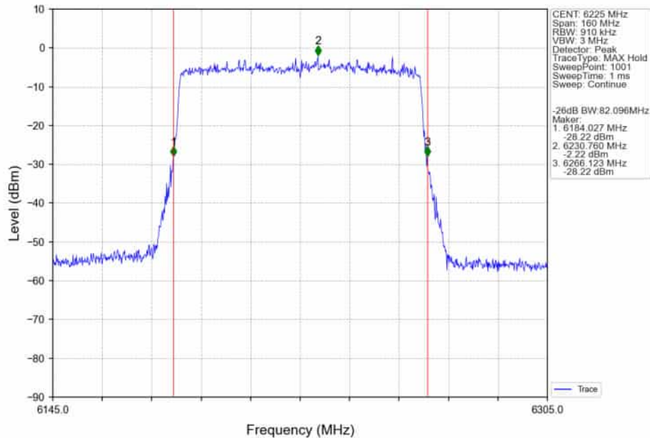
802.11ax(HEW80)_MCH_6225MHz_RU996_Left_Ant2_NTNV
