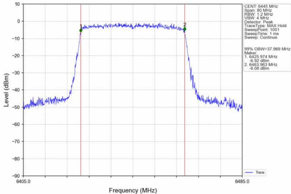
802.11ax(HEW40)_LCH_6445MHz_RU484_Left_Ant2_NTNV
