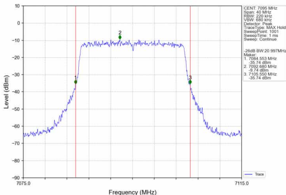
802.11ax(HEW20)_HCH_7095MHz_RU242_Left_Ant2_NTNV
