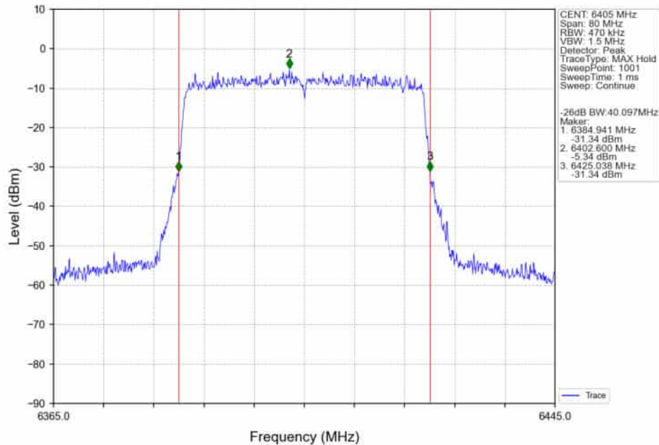
802.11ax(HEW40)_HCH_6405MHz_RU484_Left_Ant2_NTNV
