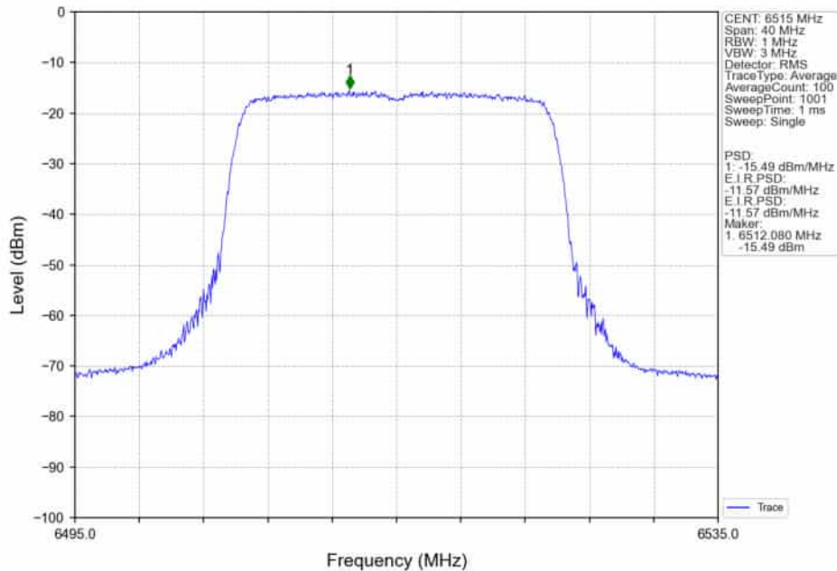
802.11ax(HEW20)_HCH_6515MHz_RU242_Left_Ant2_NTNV
