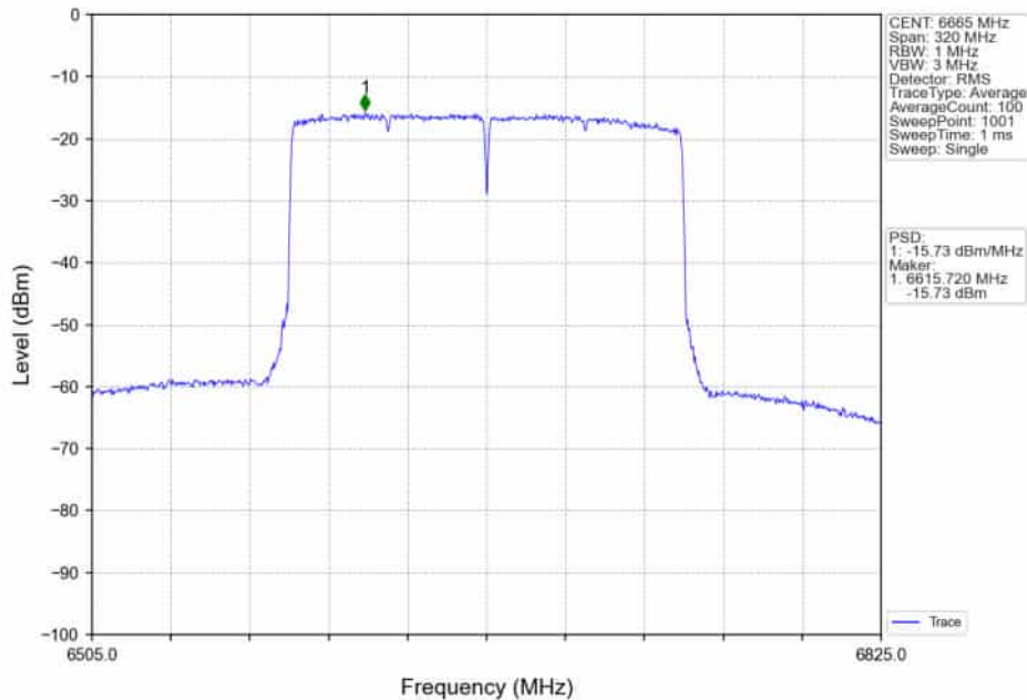
802.11ax(HEW160)_MCH_6665MHz_2xRU996_Left_MIMO_NTNV
