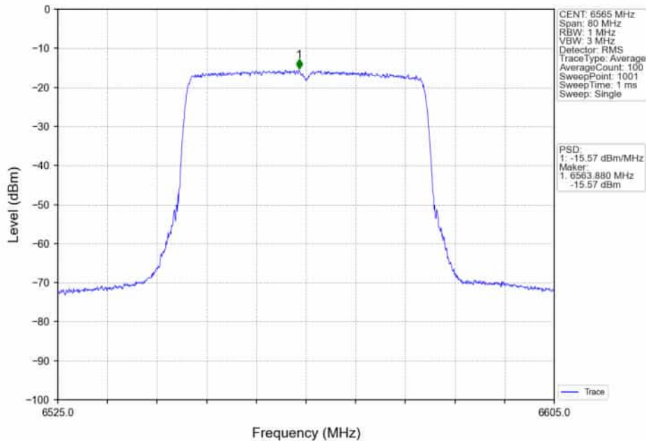
802.11ax(HEW40)_LCH_6565MHz_RU484_Left_MIMO_NTNV
