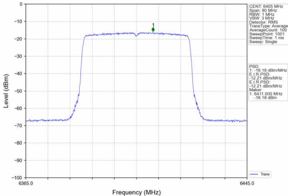
802.11ax(HEW40)_HCH_6405MHz_RU484_Left_MIMO_NTNV
