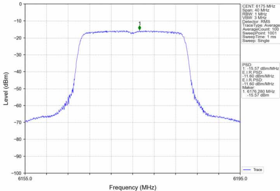
802.11ax(HEW20)_MCH_6175MHz_RU242_Left_MIMO_NTNV
