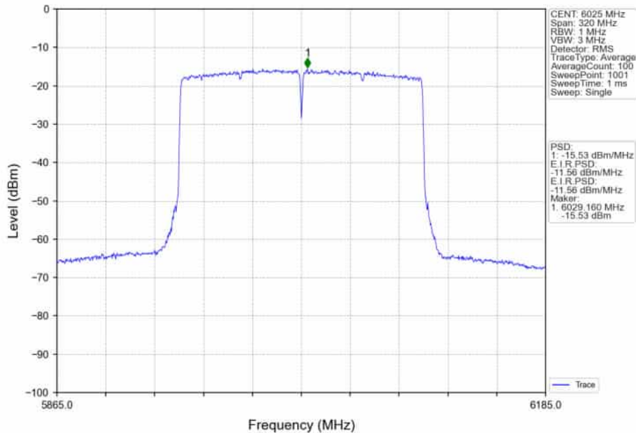
802.11ax(HEW160)_LCH_6025MHz_2xRU996_Left_MIMO_NTNV
