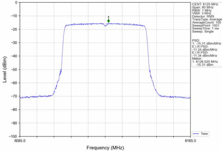
802.11ax(HEW40)_LCH_6125MHz_RU484_Left_MIMO_NTNV
