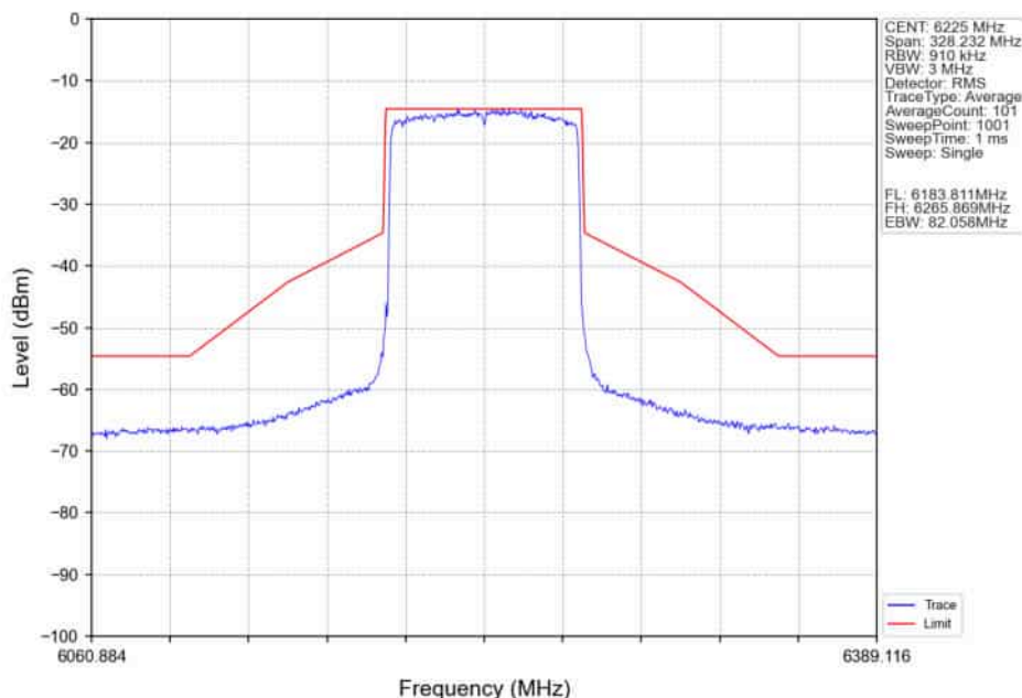
802.11ax(HEW80)_MCH_6225MHz_RU996_Left_Ant2_NTNV
