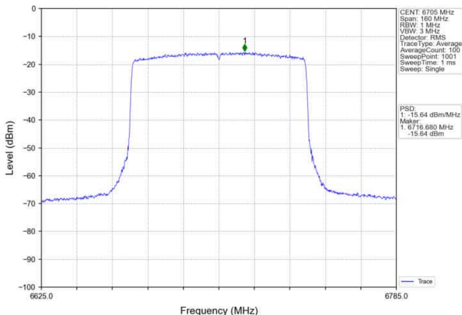
802.11ax(HEW80)_MCH_6705MHz_RU996_Left_MIMO_NTNV
