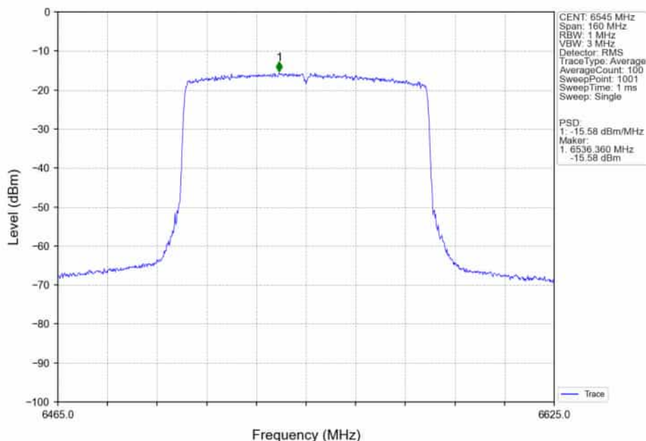
802.11ax(HEW80)_HCH_6545MHz_RU996_Left_MIMO_NTNV
