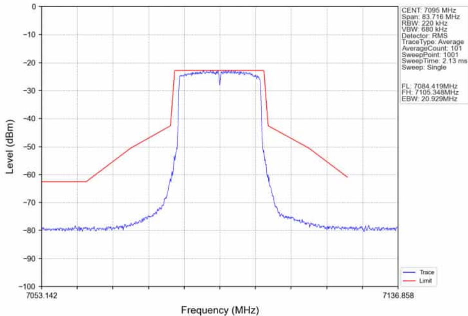
802.11ax(HEW20)_HCH_7095MHz_RU242_Left_Ant2_NTNV
