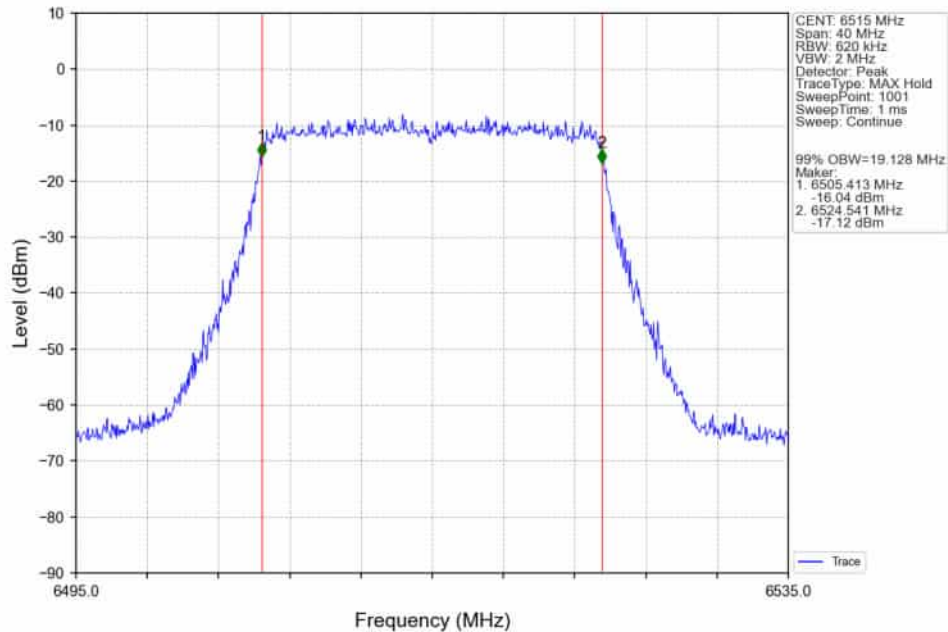
802.11ax(HEW20)_HCH_6515MHz_RU242_Left_Ant2_NTNV
