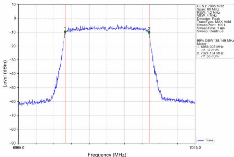
802.11ax(HEW40)_MCH_7005MHz_RU484_Left_Ant2_NTNV
