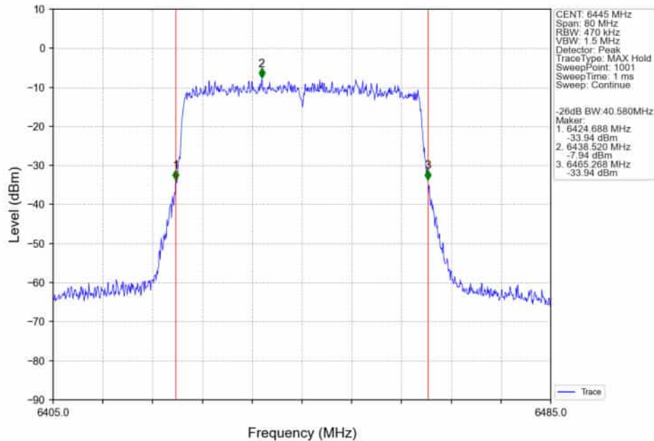
802.11ax(HEW40)_LCH_6445MHz_RU484_Left_Ant2_NTNV
