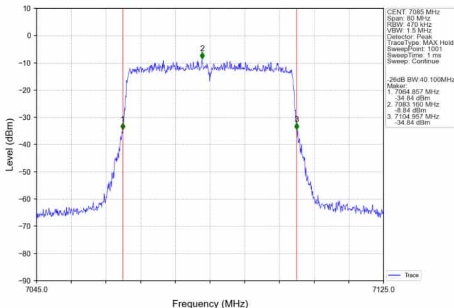
802.11ax(HEW40)_HCH_7085MHz_RU484_Left_Ant2_NTNV
