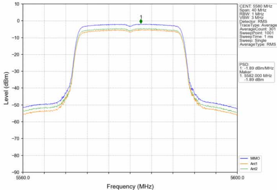
802.11ax(HE20)_MCH_5580MHz_RU242_Left_MIMO_NTNV
