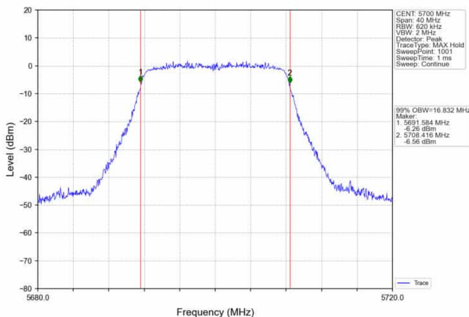
802.11a_HCH_5700MHz_Ant1_NTNV
