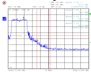
Bandedge-CH11
