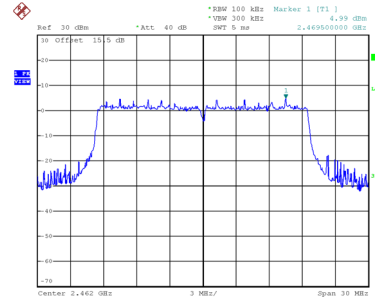
Reference Level-CH11
