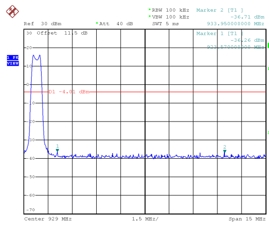
Bandedge CH02 (Upper)
