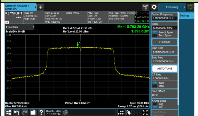
802.11ax-HE80 Power Spectral Density
