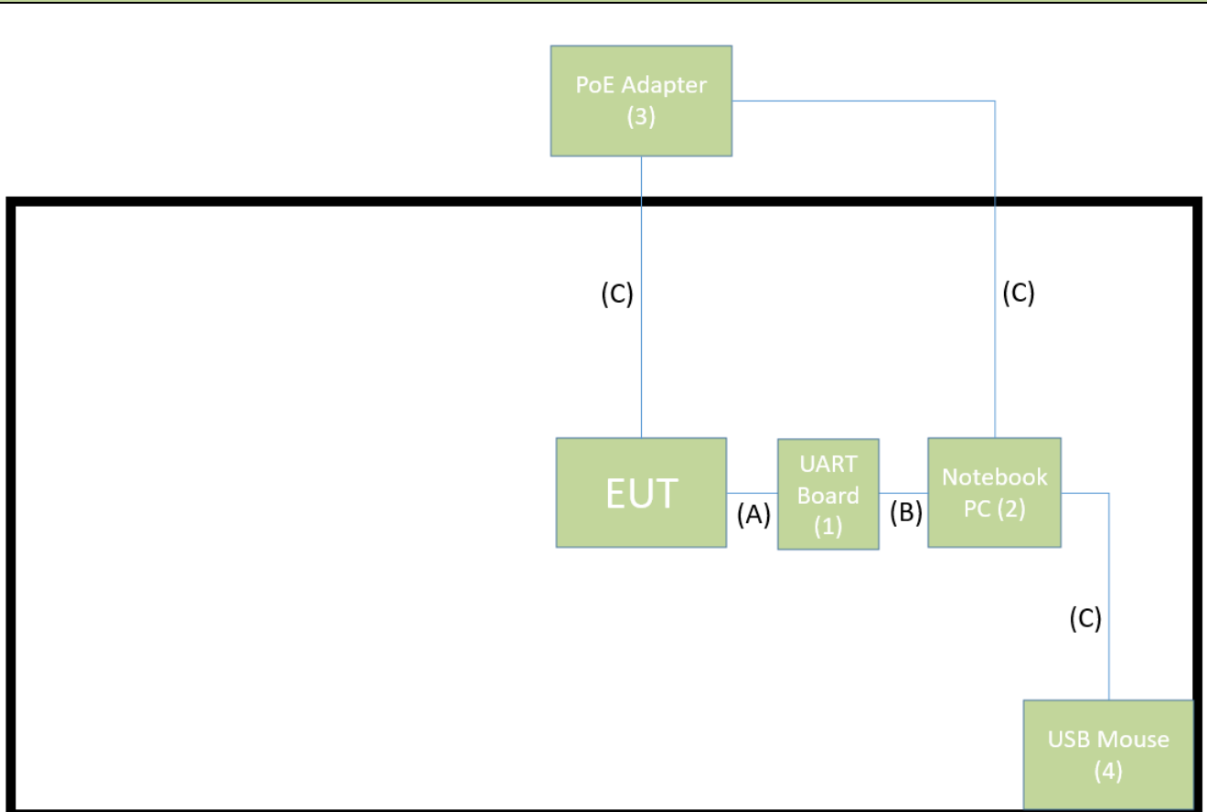
Connection Diagram
