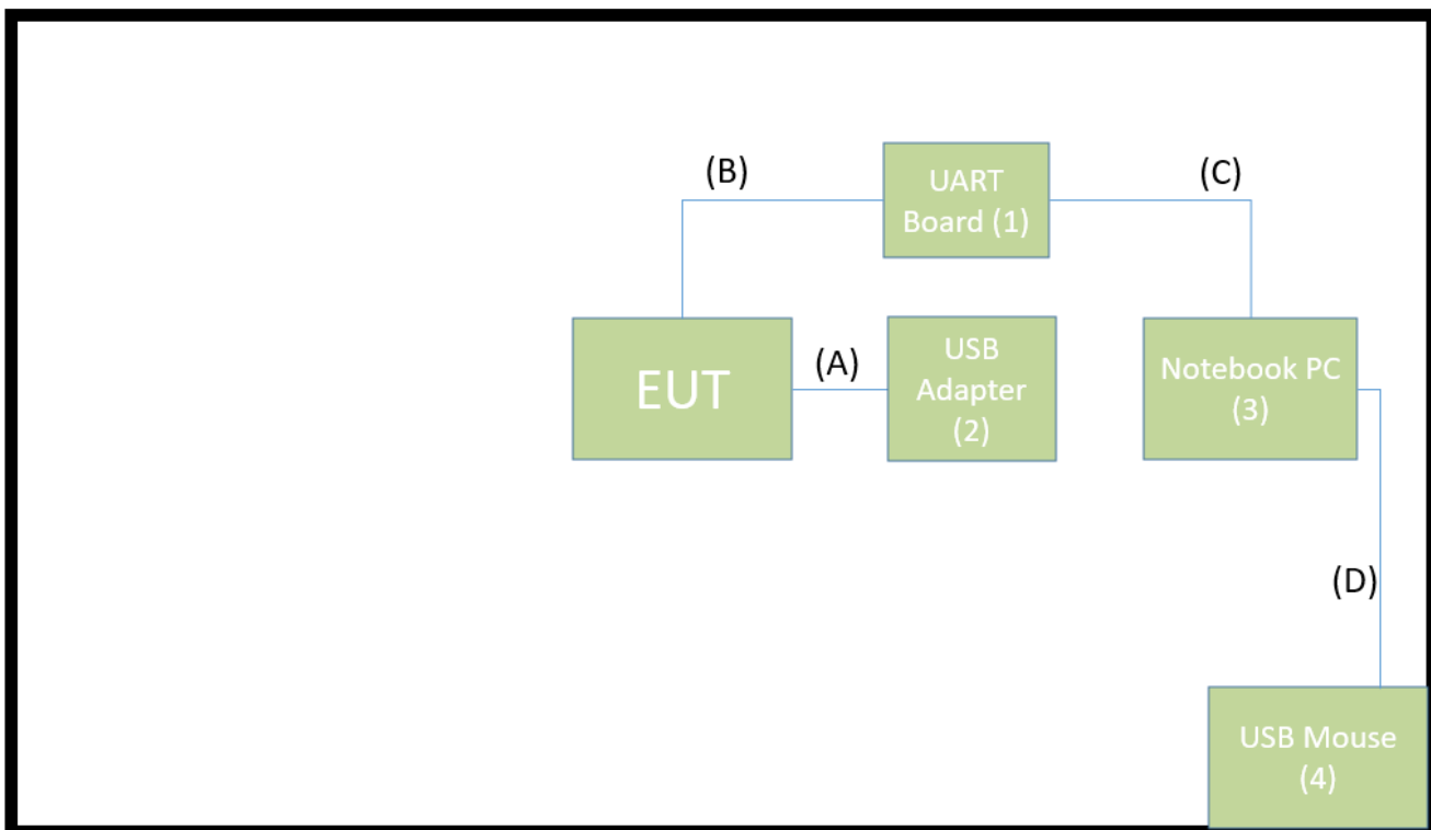
Connection Diagram
