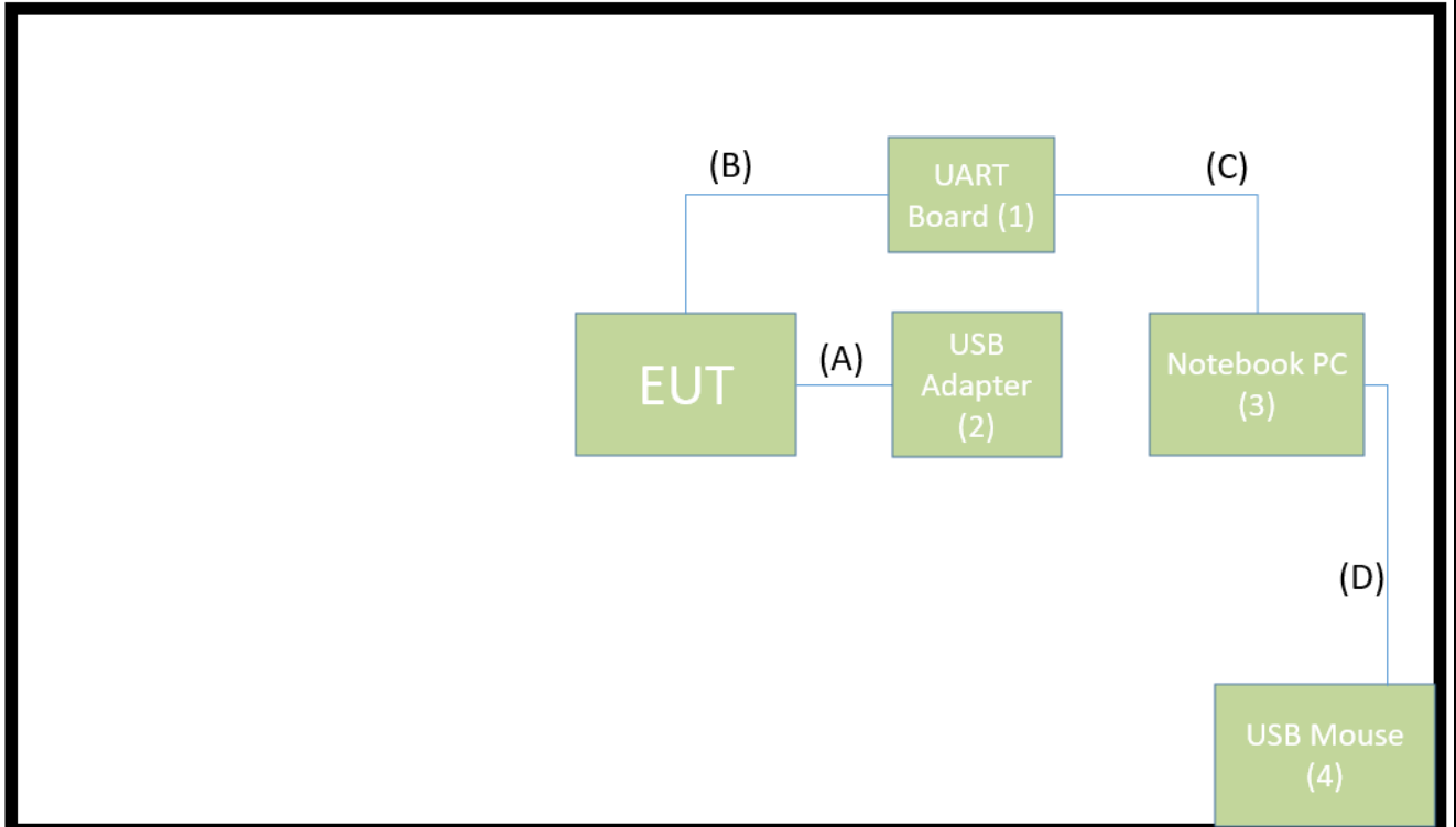
Connection Diagram
