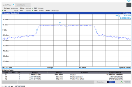
99 % Occupied Bandwidth
