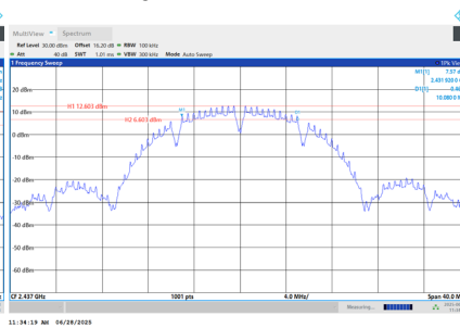
CH06 6 dB Bandwidth
