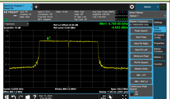
Channel 175 (6825MHz)
