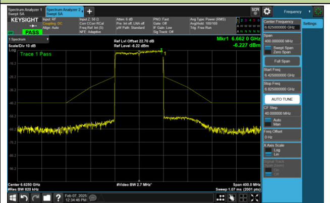
Channel 135 (6625MHz)
