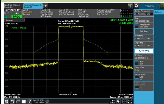
Channel 119 (6545MHz)
