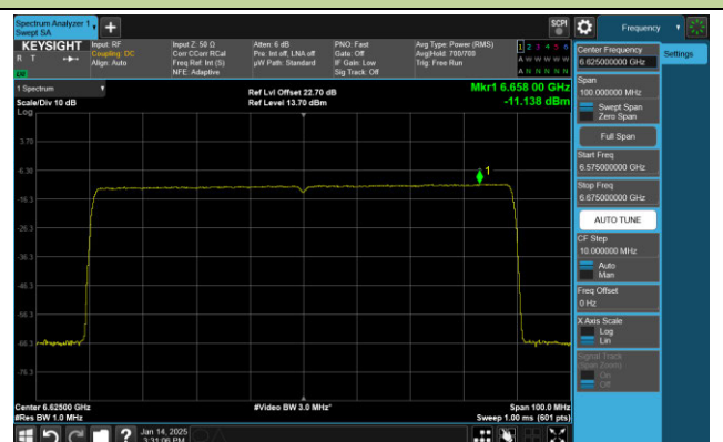
Channel 135 (6625MHz)
