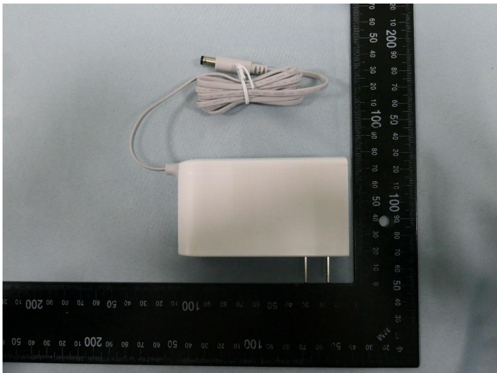
(8) EUT Photo (Brand: tp-link, M/N: T120200-2B4)
