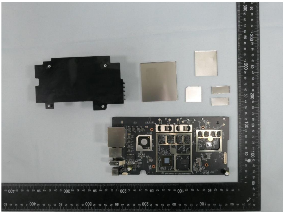
(35) EUT Photo
