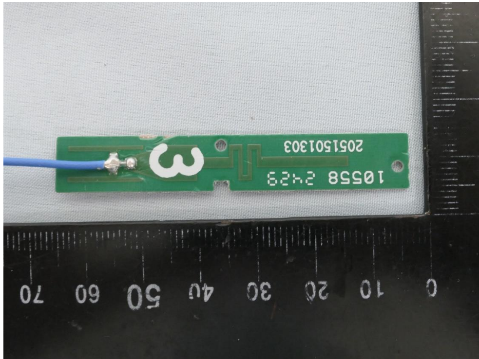
(26) EUT Photo
