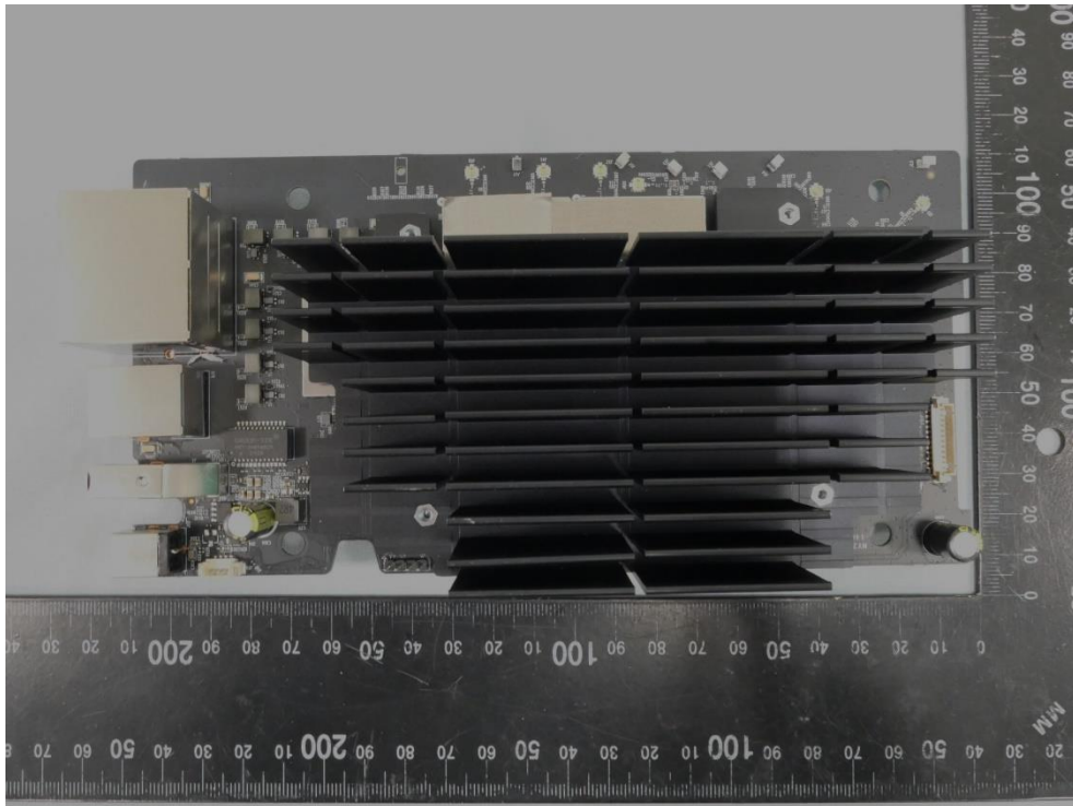
(34) EUT Photo
