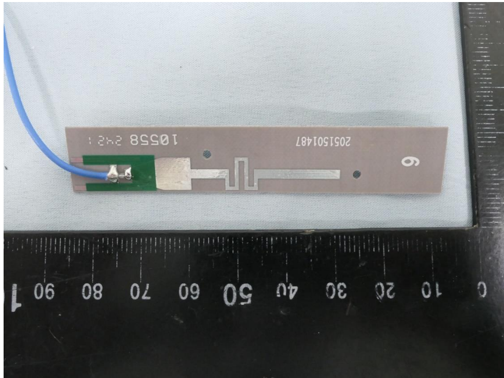
(32) EUT Photo
