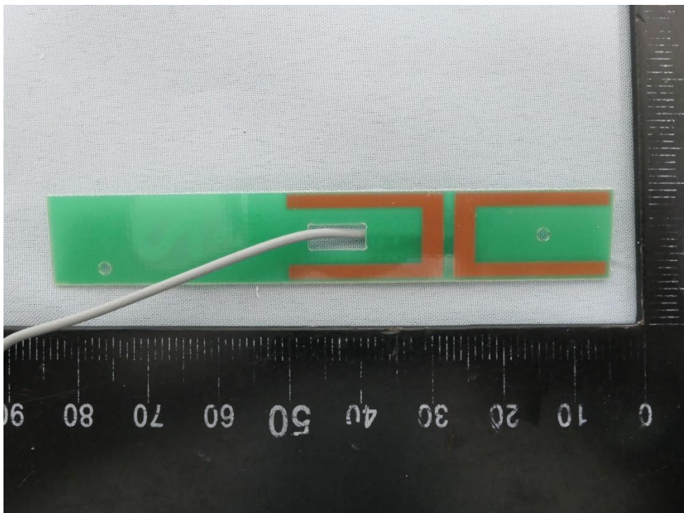
(25) EUT Photo
