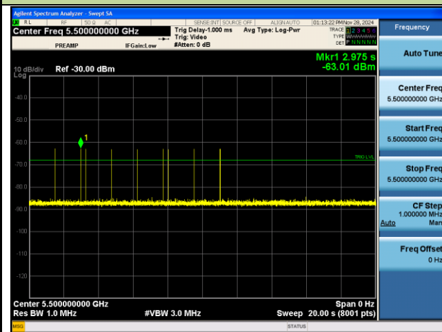
Radars #5
