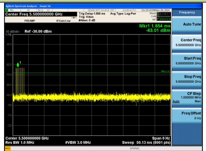
Radars #6
