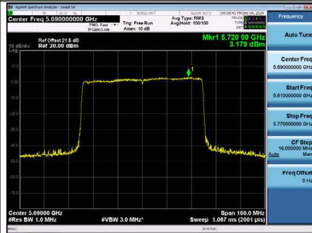
802.11be-EHT160 Power Spectral Density - Ant 1
