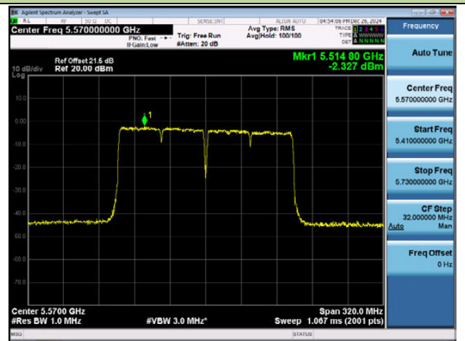
Channel 114 (5570MHz)
