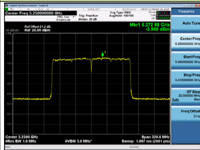
Channel 50 (5250MHz)
