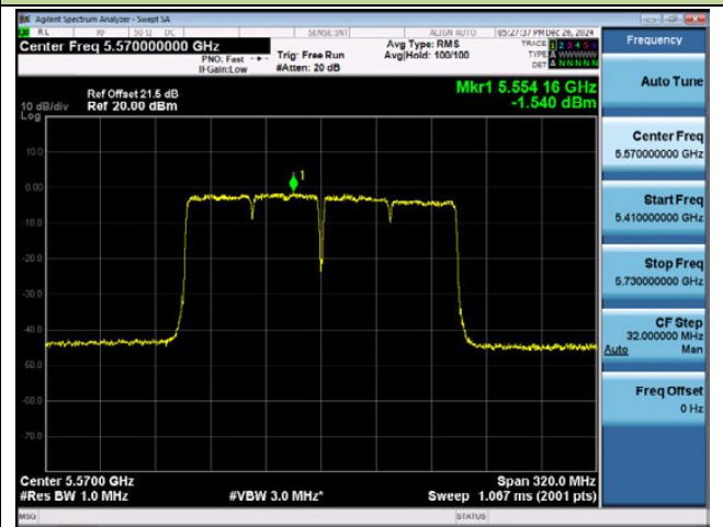
Channel 114 (5570MHz)
