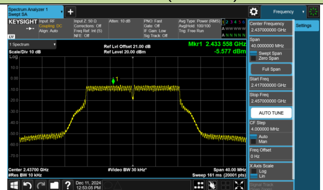
Channel 06 (2437MHz)
