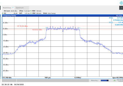
CH157 6 dB Bandwidth
