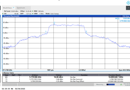
99 % Occupied Bandwidth
