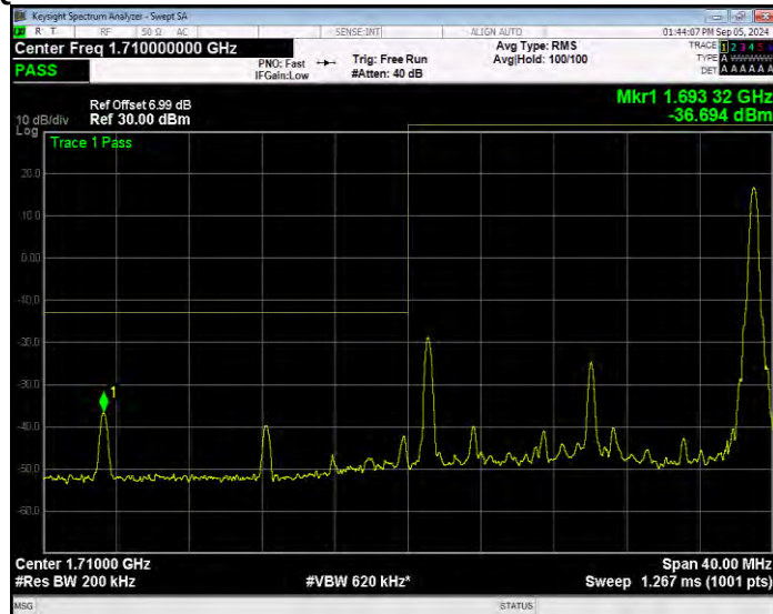
Band4 16QAM BW=20MHz Channel=20050 RB Size=27 Position=#0 Extended
