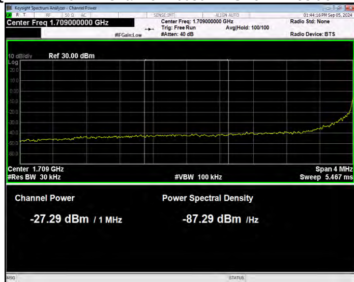
Band4 16QAM BW=20MHz Channel=20050 RB Size=27 Position=#0 Normal
