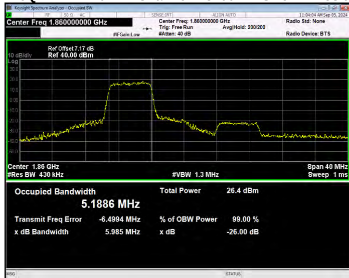
Band2 16QAM BW=20MHz Channel=18900 RB Size=27 Position=#0
