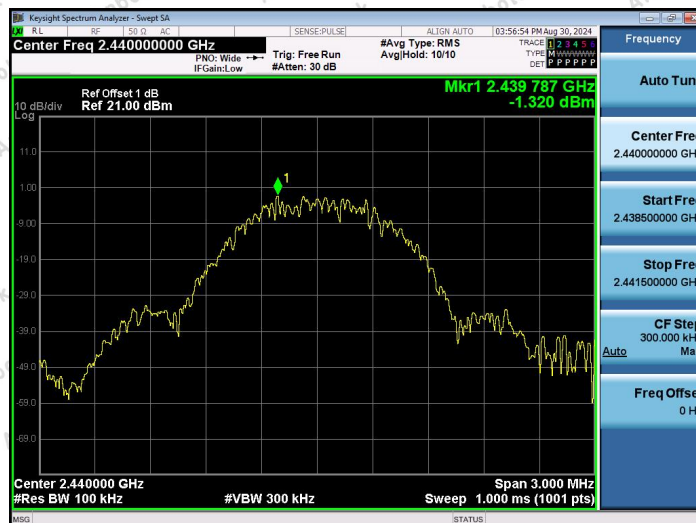
2.4G-Ant1-2440-0~Reference-PASS
