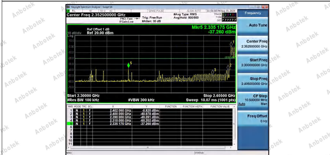
DH5-Ant1-Hop_2402-PASS
