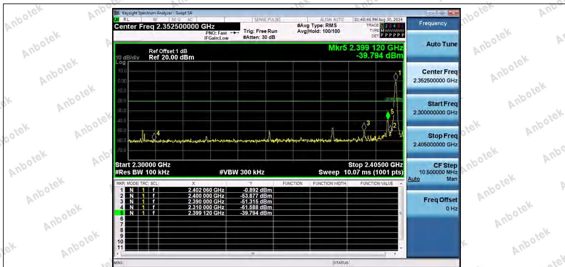
DH5-Ant1-2402-PASS
