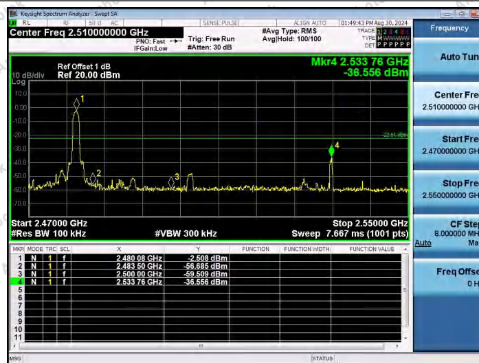
2DH5-Ant1-2480-PASS
