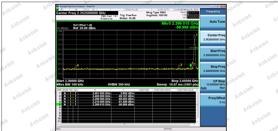
2.4G-Ant1-2402-PASS
