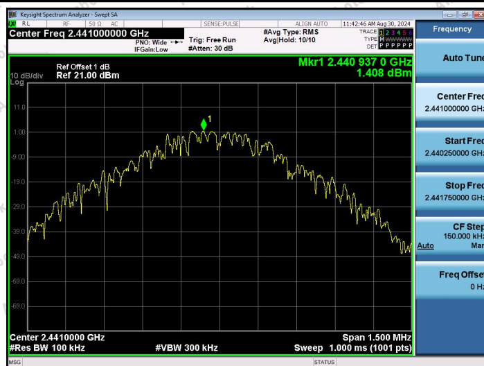
2.4G-Ant1-2441-0~Reference-PASS
