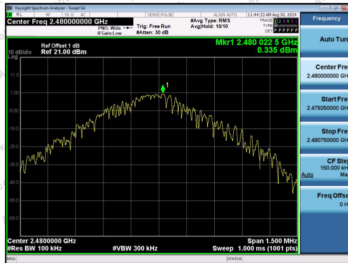
2.4G-Ant1-2480-0~Reference-PASS
