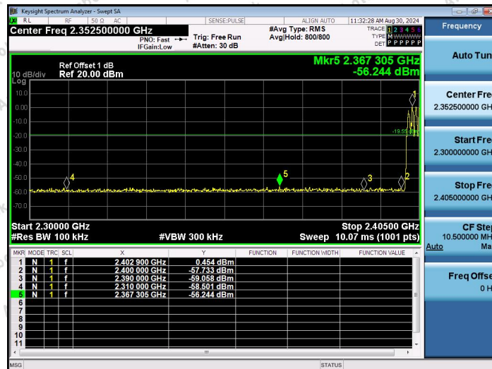
2.4G-Ant1-Hop_2402-PASS
