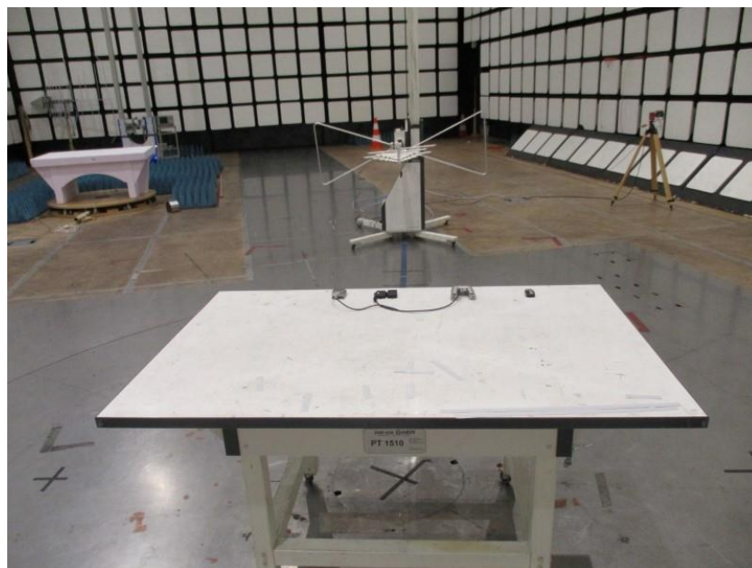
Picture 2: Radiated disturbance 30M-1GHz
