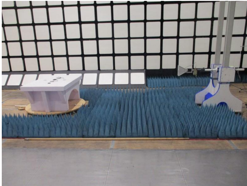
Picture 5: Radiated disturbance >1GHz
