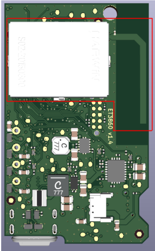
Picture 5 :Radio Module location image & Antenna Location
