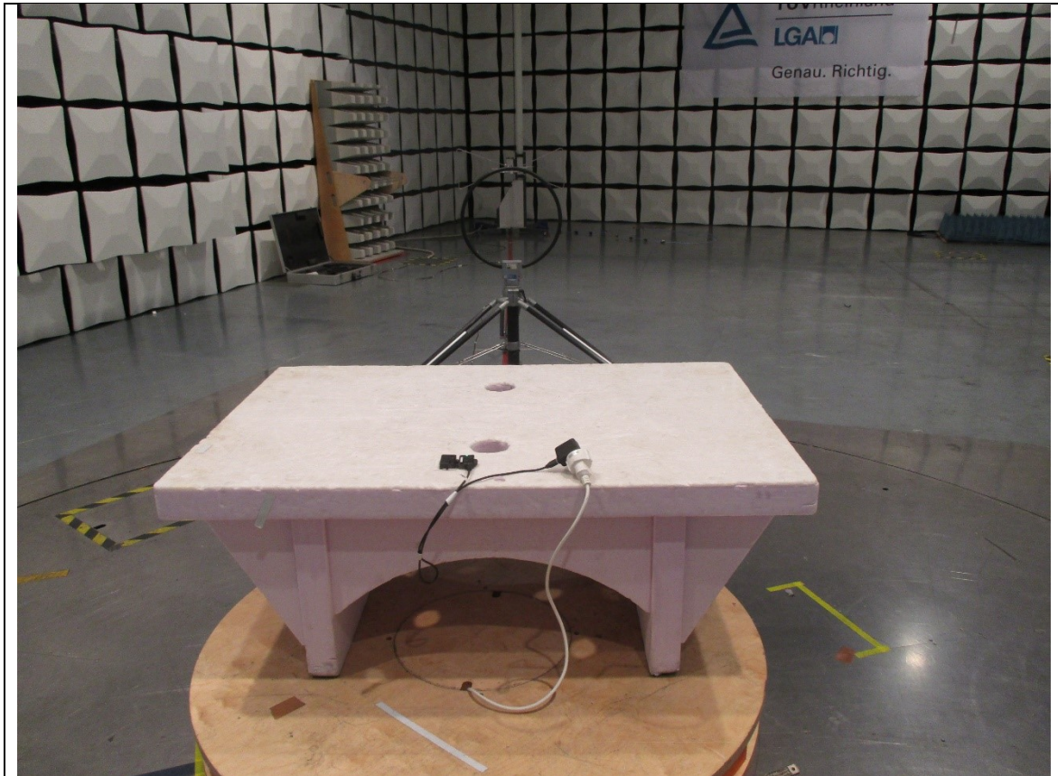
Test Setup: Radiated Measurements (9 kHz - 30 MHz)
