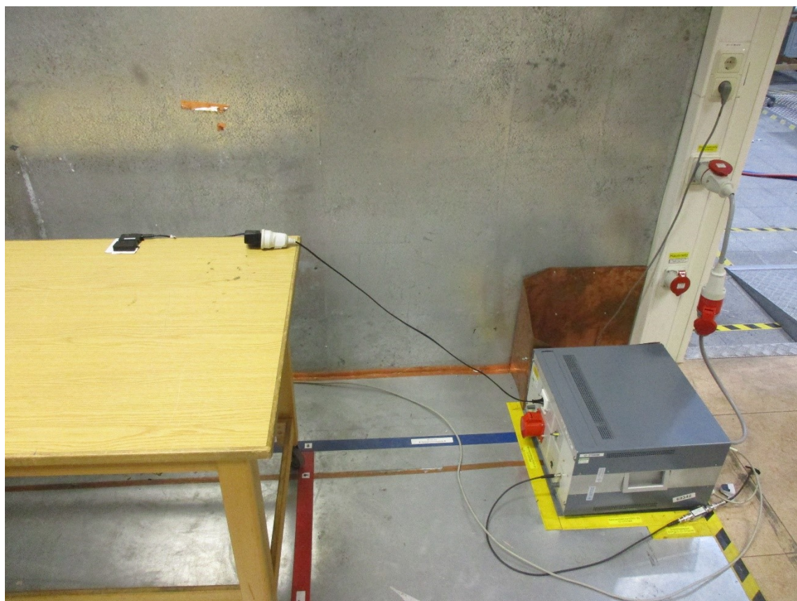
Test Setup: Conducted Emission Measurements
