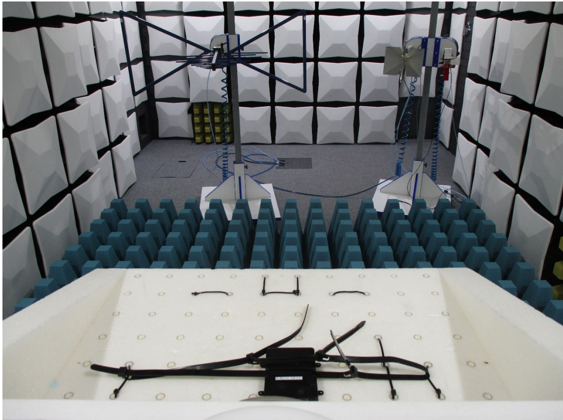
Test Setup: Radiated Measurements (1 GHz to 26 GHz)
