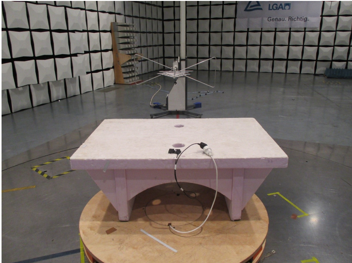
Test Setup: Radiated Measurements (30 MHz - 1 GHz)
